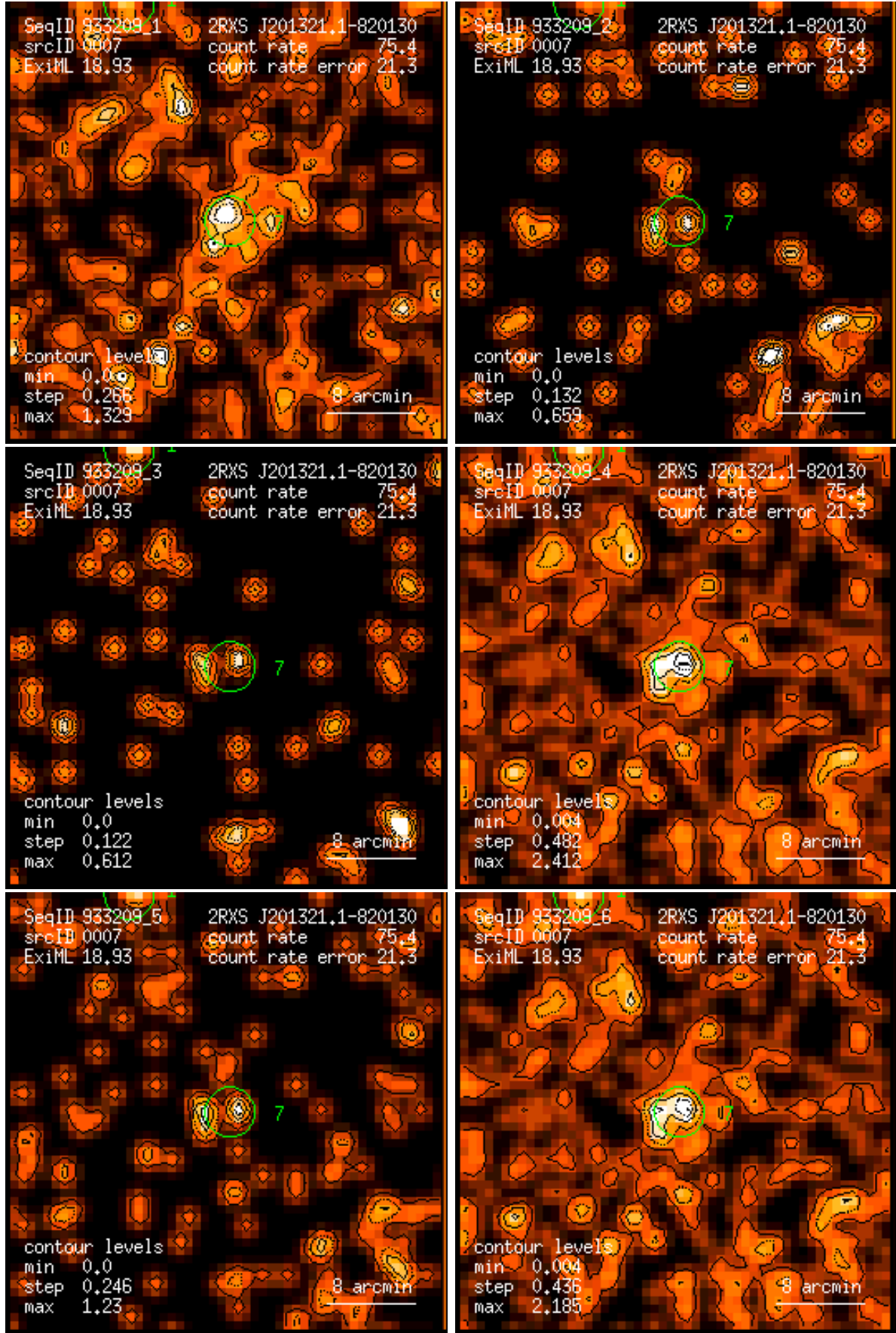
Figure 7: RASS 933209: detection 0007: band rate images, Gaussian filter: (1) PSPC channels 11 – 41, (2) 52 – 90, (3) 91 – 201, (4) 11 – 235, (5) 52 – 201, (6) 11 – 201. Broad band rates in counts/ks. Band rate contour levels in counts/ks/arcmin 2 .
