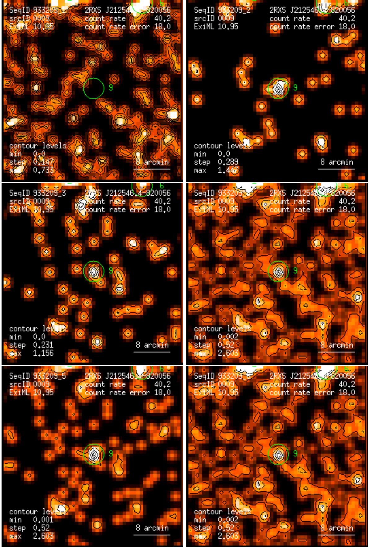
Figure 9: RASS 933209: detection 0009: band rate images, Gaussian filter: (1) PSPC channels 11 – 41, (2) 52 – 90, (3) 91 – 201, (4) 11 – 235, (5) 52 – 201, (6) 11 – 201. Broad band rates in counts/ks. Band rate contour levels in counts/ks/arcmin 2 .
