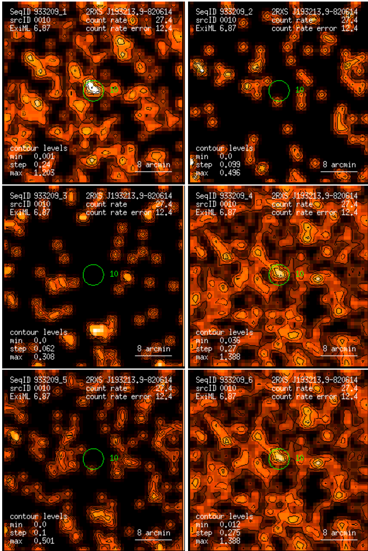
Figure 10: RASS 933209: detection 0010: band rate images, Gaussian filter: (1) PSPC channels 11 – 41, (2) 52 – 90, (3) 91 – 201, (4) 11 – 235, (5) 52 – 201, (6) 11 – 201. Broad band rates in counts/ks. Band rate contour levels in counts/ks/arcmin 2 .
