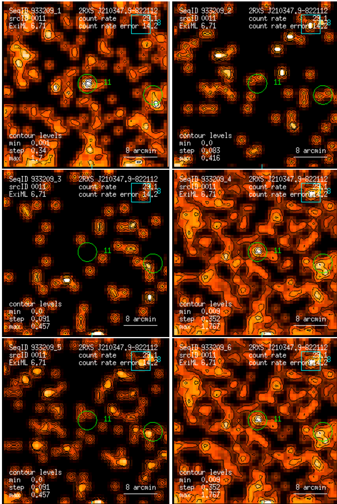
Figure 11: RASS 933209: detection 0011: band rate images, Gaussian filter: (1) PSPC channels 11 – 41, (2) 52 – 90, (3) 91 – 201, (4) 11 – 235, (5) 52 – 201, (6) 11 – 201. Broad band rates in counts/ks. Band rate contour levels in counts/ks/arcmin 2 .
