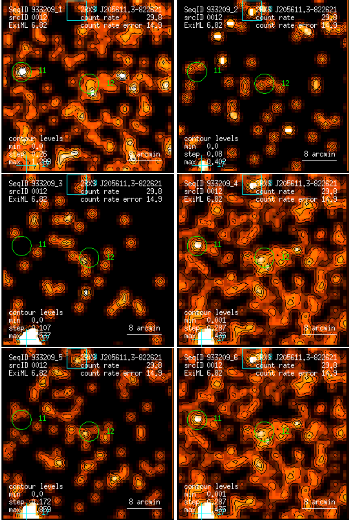
Figure 12: RASS 933209: detection 0012: band rate images, Gaussian filter: (1) PSPC channels 11 – 41, (2) 52 – 90, (3) 91 – 201, (4) 11 – 235, (5) 52 – 201, (6) 11 – 201. Broad band rates in counts/ks. Band rate contour levels in counts/ks/arcmin 2 .
