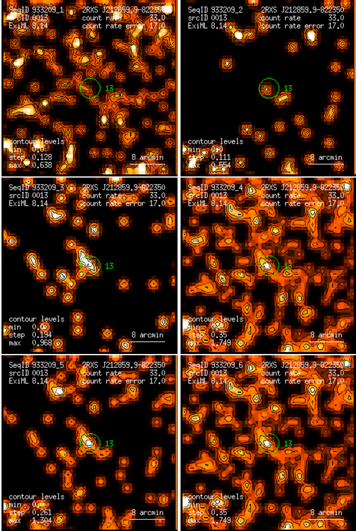
Figure 13: RASS 933209: detection 0013: band rate images, Gaussian filter: (1) PSPC channels 11 – 41, (2) 52 – 90, (3) 91 – 201, (4) 11 – 235, (5) 52 – 201, (6) 11 – 201. Broad band rates in counts/ks. Band rate contour levels in counts/ks/arcmin 2 .
