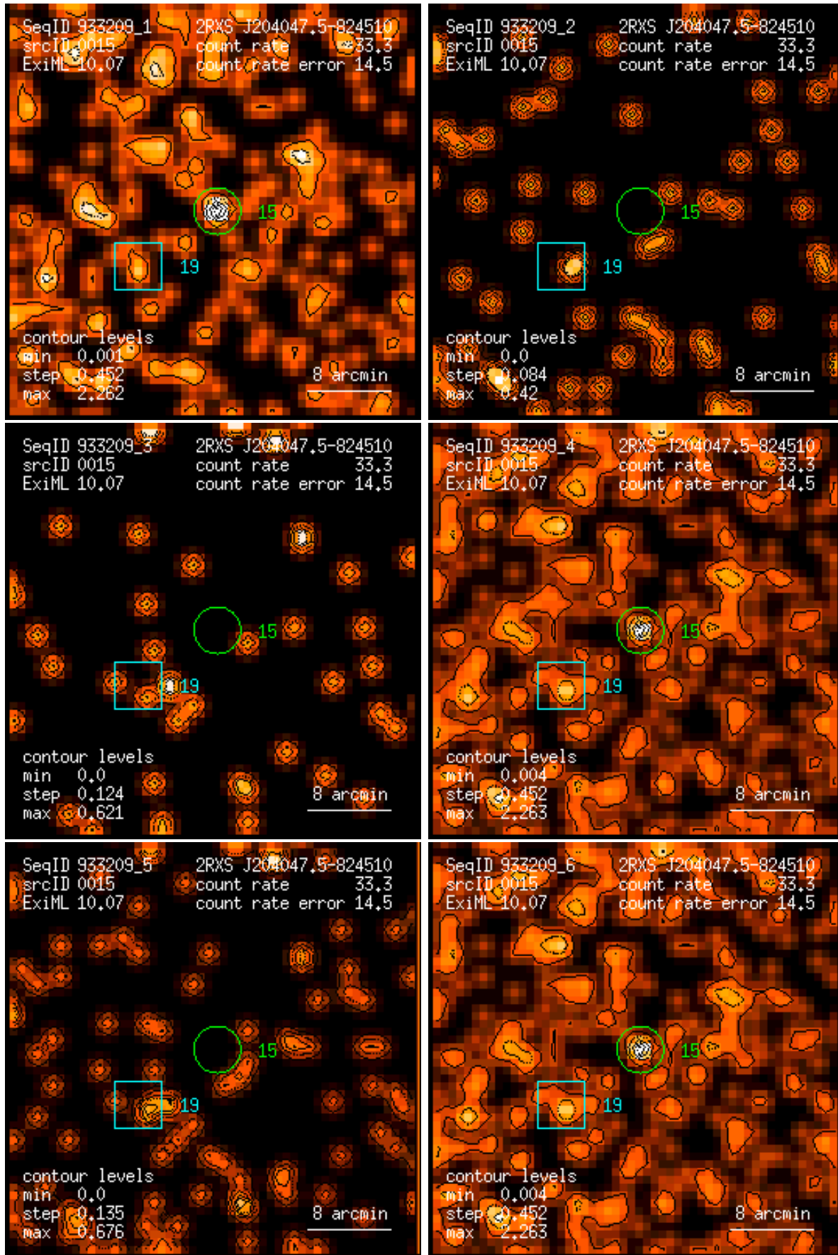
Figure 15: RASS 933209: detection 0015: band rate images, Gaussian filter: (1) PSPC channels 11 – 41, (2) 52 – 90, (3) 91 – 201, (4) 11 – 235, (5) 52 – 201, (6) 11 – 201. Broad band rates in counts/ks. Band rate contour levels in counts/ks/arcmin 2 .
