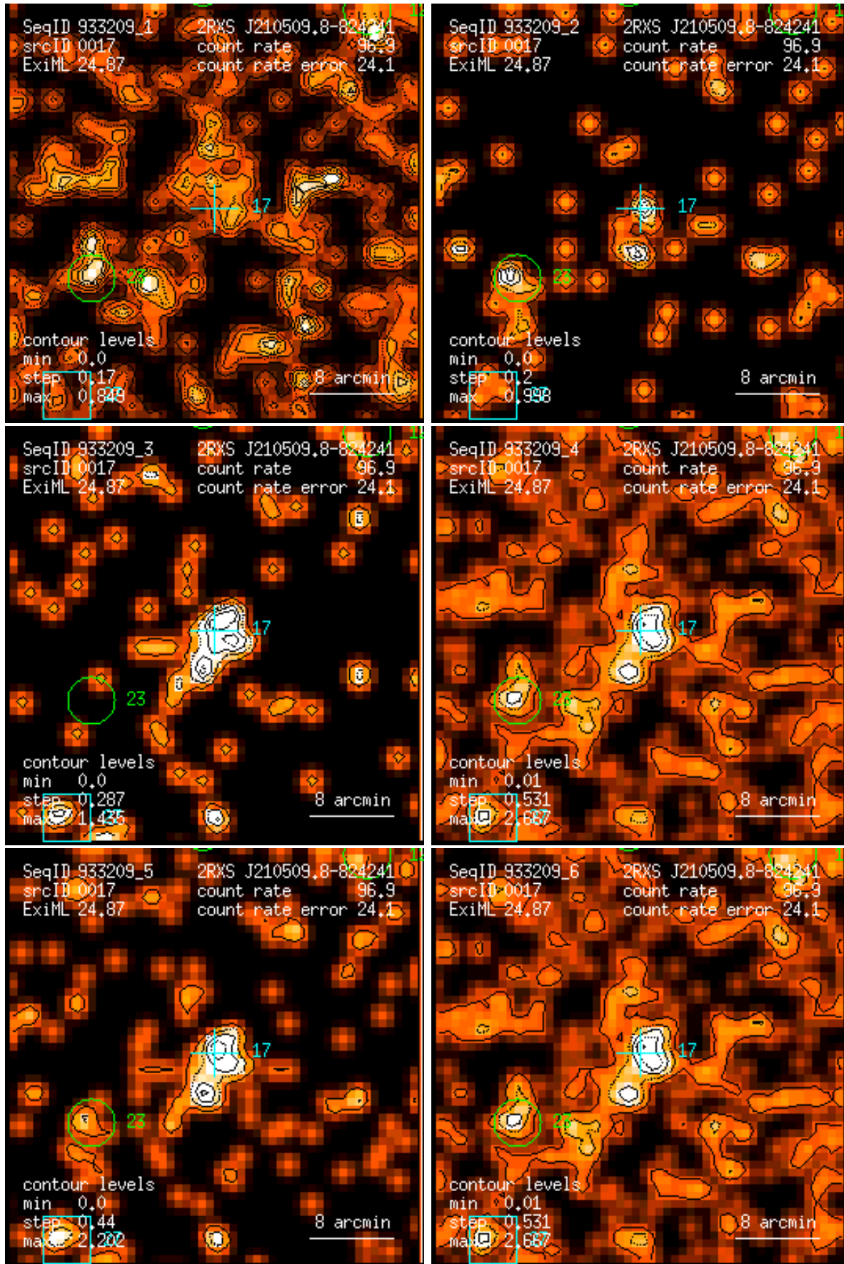
Figure 17: RASS 933209: detection 0017: band rate images, Gaussian filter: (1) PSPC channels 11 – 41, (2) 52 – 90, (3) 91 – 201, (4) 11 – 235, (5) 52 – 201, (6) 11 – 201. Broad band rates in counts/ks. Band rate contour levels in counts/ks/arcmin 2 .
