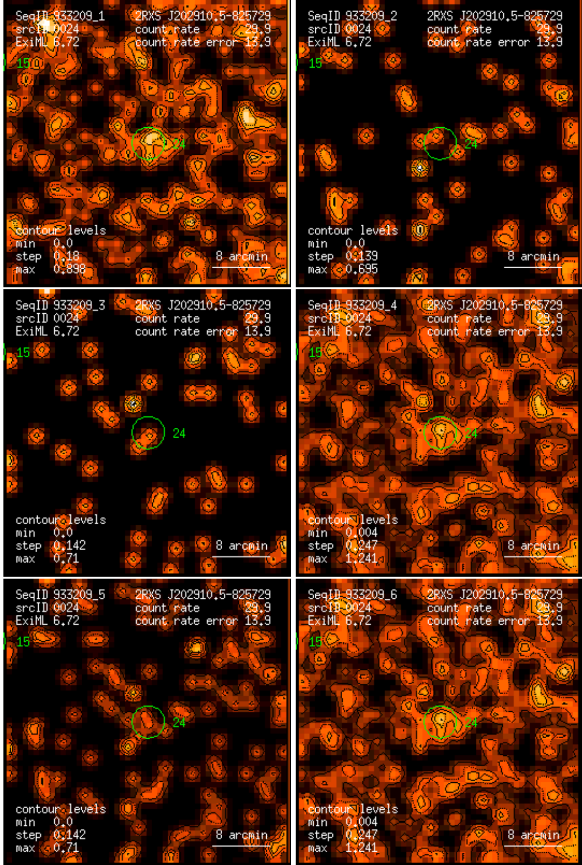
Figure 24: RASS 933209: detection 0024: band rate images, Gaussian filter: (1) PSPC channels 11 – 41, (2) 52 – 90, (3) 91 – 201, (4) 11 – 235, (5) 52 – 201, (6) 11 – 201. Broad band rates in counts/ks. Band rate contour levels in counts/ks/arcmin 2 .
