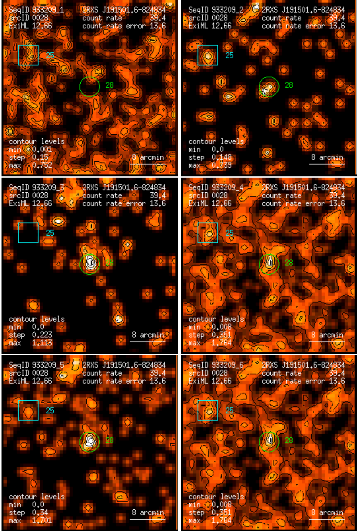
Figure 28: RASS 933209: detection 0028: band rate images, Gaussian filter: (1) PSPC channels 11 – 41, (2) 52 – 90, (3) 91 – 201, (4) 11 – 235, (5) 52 – 201, (6) 11 – 201. Broad band rates in counts/ks. Band rate contour levels in counts/ks/arcmin 2 .
