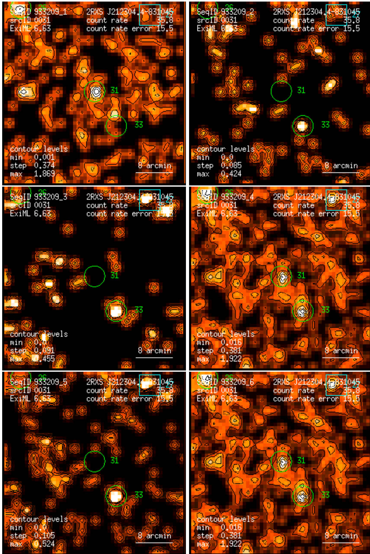
Figure 31: RASS 933209: detection 0031: band rate images, Gaussian filter: (1) PSPC channels 11 – 41, (2) 52 – 90, (3) 91 – 201, (4) 11 – 235, (5) 52 – 201, (6) 11 – 201. Broad band rates in counts/ks. Band rate contour levels in counts/ks/arcmin 2 .
