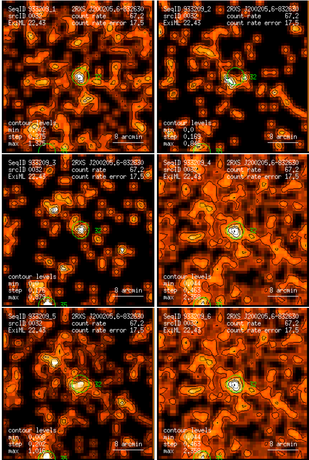
Figure 32: RASS 933209: detection 0032: band rate images, Gaussian filter: (1) PSPC channels 11 – 41, (2) 52 – 90, (3) 91 – 201, (4) 11 – 235, (5) 52 – 201, (6) 11 – 201. Broad band rates in counts/ks. Band rate contour levels in counts/ks/arcmin 2 .
