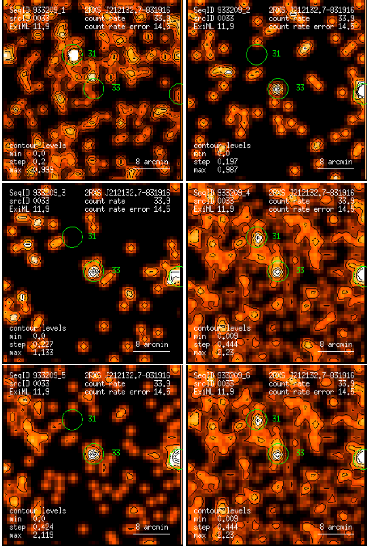
Figure 33: RASS 933209: detection 0033: band rate images, Gaussian filter: (1) PSPC channels 11 – 41, (2) 52 – 90, (3) 91 – 201, (4) 11 – 235, (5) 52 – 201, (6) 11 – 201. Broad band rates in counts/ks. Band rate contour levels in counts/ks/arcmin 2 .
