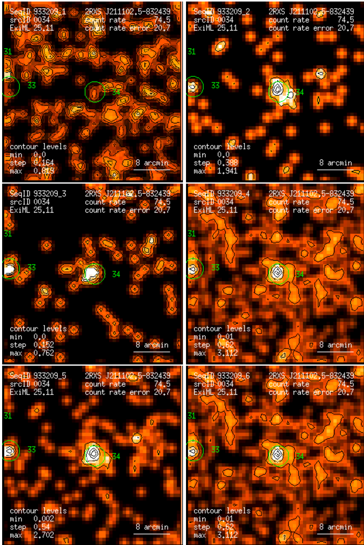
Figure 34: RASS 933209: detection 0034: band rate images, Gaussian filter: (1) PSPC channels 11 – 41, (2) 52 – 90, (3) 91 – 201, (4) 11 – 235, (5) 52 – 201, (6) 11 – 201. Broad band rates in counts/ks. Band rate contour levels in counts/ks/arcmin 2 .
