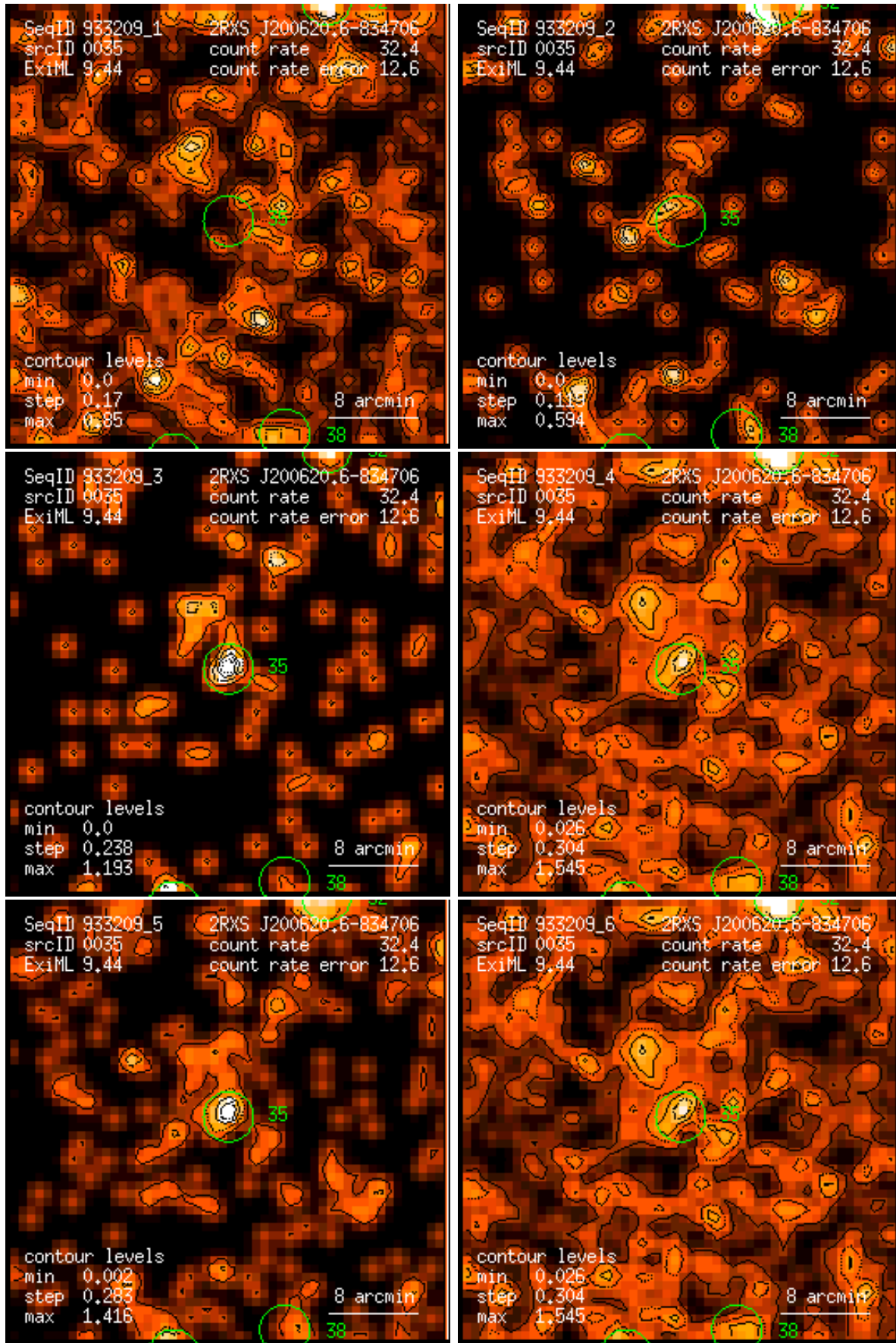
Figure 35: RASS 933209: detection 0035: band rate images, Gaussian filter: (1) PSPC channels 11 – 41, (2) 52 – 90, (3) 91 – 201, (4) 11 – 235, (5) 52 – 201, (6) 11 – 201. Broad band rates in counts/ks. Band rate contour levels in counts/ks/arcmin 2 .
