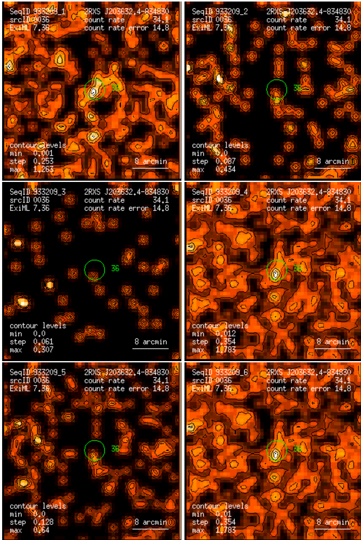
Figure 36: RASS 933209: detection 0036: band rate images, Gaussian filter: (1) PSPC channels 11 – 41, (2) 52 – 90, (3) 91 – 201, (4) 11 – 235, (5) 52 – 201, (6) 11 – 201. Broad band rates in counts/ks. Band rate contour levels in counts/ks/arcmin 2 .
