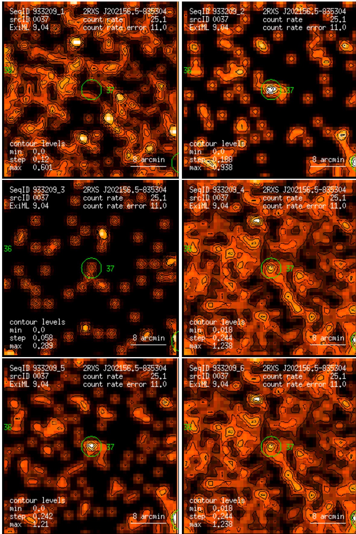
Figure 37: RASS 933209: detection 0037: band rate images, Gaussian filter: (1) PSPC channels 11 – 41, (2) 52 – 90, (3) 91 – 201, (4) 11 – 235, (5) 52 – 201, (6) 11 – 201. Broad band rates in counts/ks. Band rate contour levels in counts/ks/arcmin 2 .
