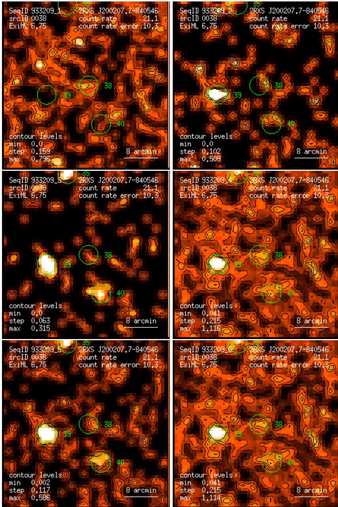
Figure 38: RASS 933209: detection 0038: band rate images, Gaussian filter: (1) PSPC channels 11 – 41, (2) 52 – 90, (3) 91 – 201, (4) 11 – 235, (5) 52 – 201, (6) 11 – 201. Broad band rates in counts/ks. Band rate contour levels in counts/ks/arcmin 2 .
