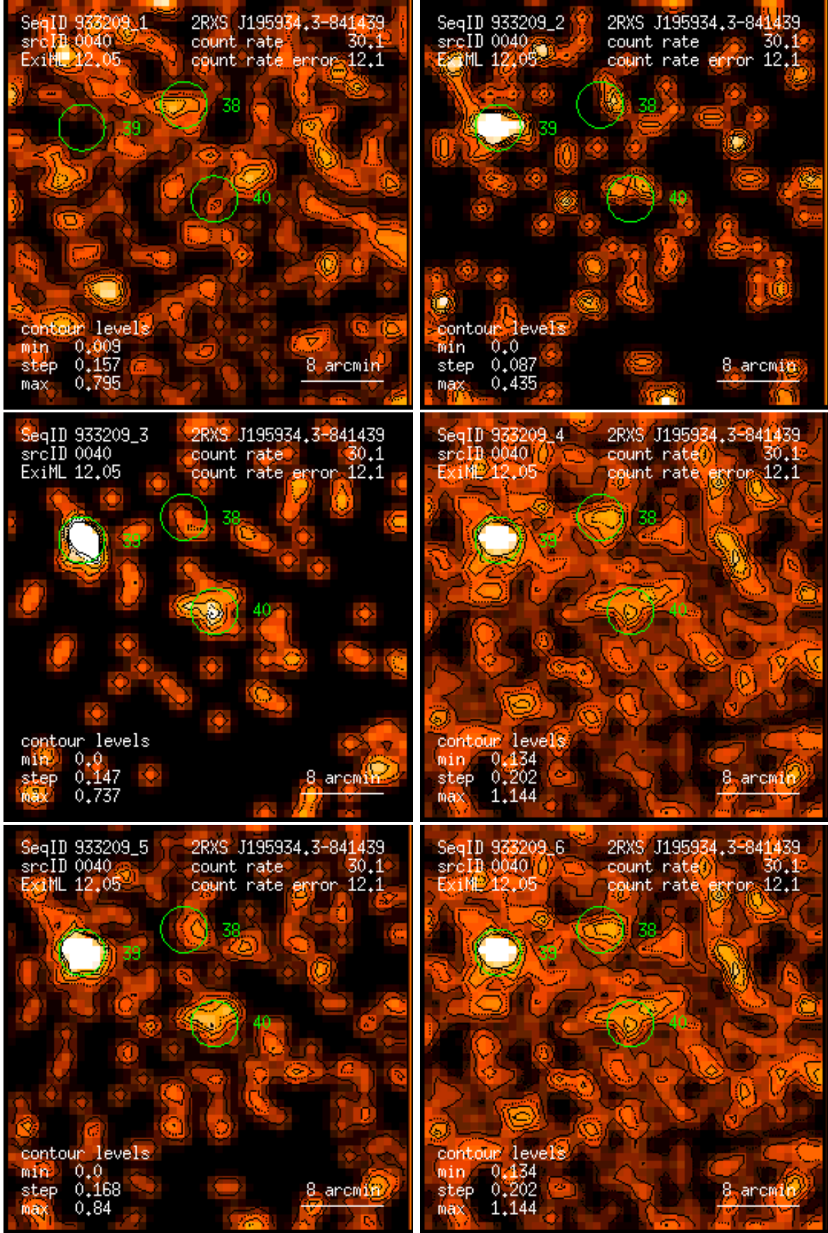
Figure 40: RASS 933209: detection 0040: band rate images, Gaussian filter: (1) PSPC channels 11 – 41, (2) 52 – 90, (3) 91 – 201, (4) 11 – 235, (5) 52 – 201, (6) 11 – 201. Broad band rates in counts/ks. Band rate contour levels in counts/ks/arcmin 2 .
