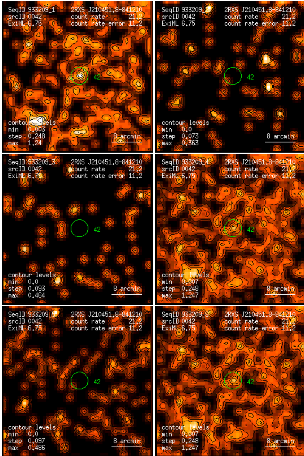
Figure 42: RASS 933209: detection 0042: band rate images, Gaussian filter: (1) PSPC channels 11 – 41, (2) 52 – 90, (3) 91 – 201, (4) 11 – 235, (5) 52 – 201, (6) 11 – 201. Broad band rates in counts/ks. Band rate contour levels in counts/ks/arcmin 2 .
