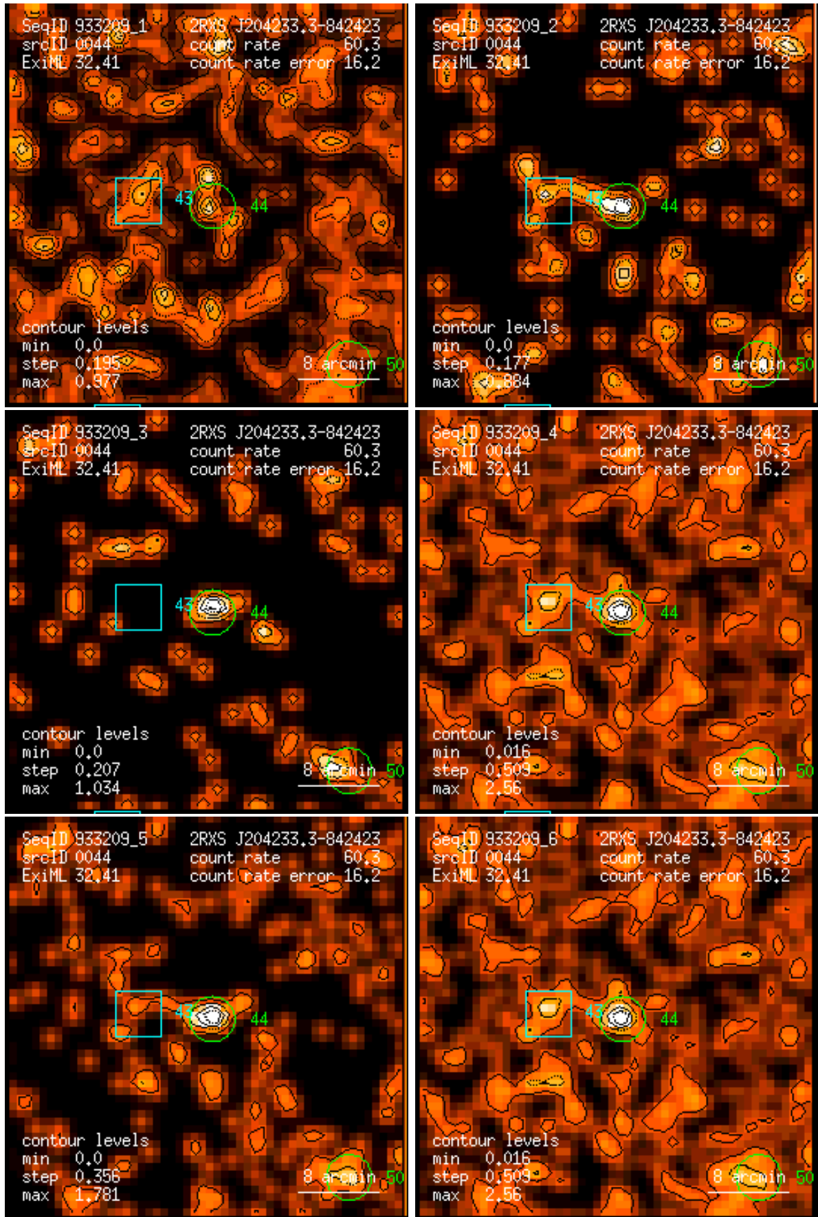
Figure 44: RASS 933209: detection 0044: band rate images, Gaussian filter: (1) PSPC channels 11 – 41, (2) 52 – 90, (3) 91 – 201, (4) 11 – 235, (5) 52 – 201, (6) 11 – 201. Broad band rates in counts/ks. Band rate contour levels in counts/ks/arcmin 2 .
