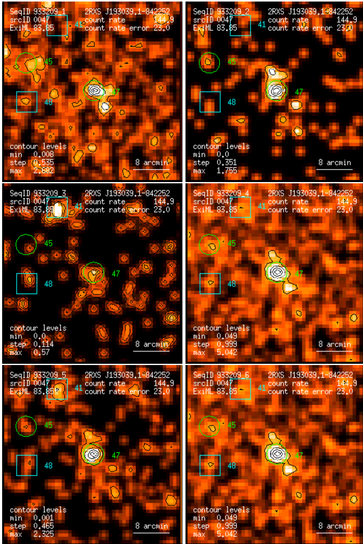
Figure 47: RASS 933209: detection 0047: band rate images, Gaussian filter: (1) PSPC channels 11 – 41, (2) 52 – 90, (3) 91 – 201, (4) 11 – 235, (5) 52 – 201, (6) 11 – 201. Broad band rates in counts/ks. Band rate contour levels in counts/ks/arcmin 2 .
