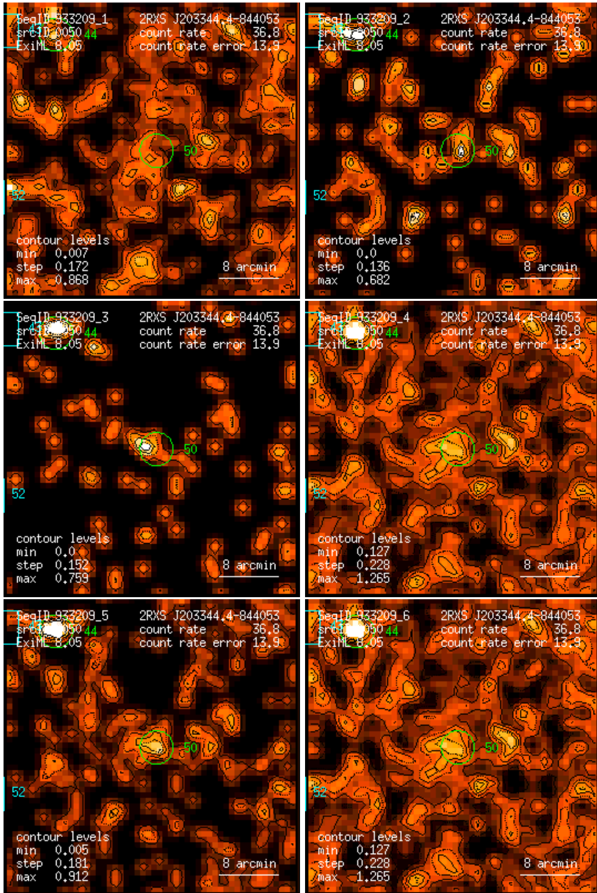
Figure 50: RASS 933209: detection 0050: band rate images, Gaussian filter: (1) PSPC channels 11 – 41, (2) 52 – 90, (3) 91 – 201, (4) 11 – 235, (5) 52 – 201, (6) 11 – 201. Broad band rates in counts/ks. Band rate contour levels in counts/ks/arcmin 2 .
