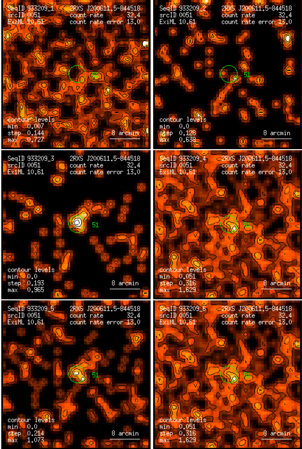
Figure 51: RASS 933209: detection 0051: band rate images, Gaussian filter: (1) PSPC channels 11 – 41, (2) 52 – 90, (3) 91 – 201, (4) 11 – 235, (5) 52 – 201, (6) 11 – 201. Broad band rates in counts/ks. Band rate contour levels in counts/ks/arcmin 2 .
