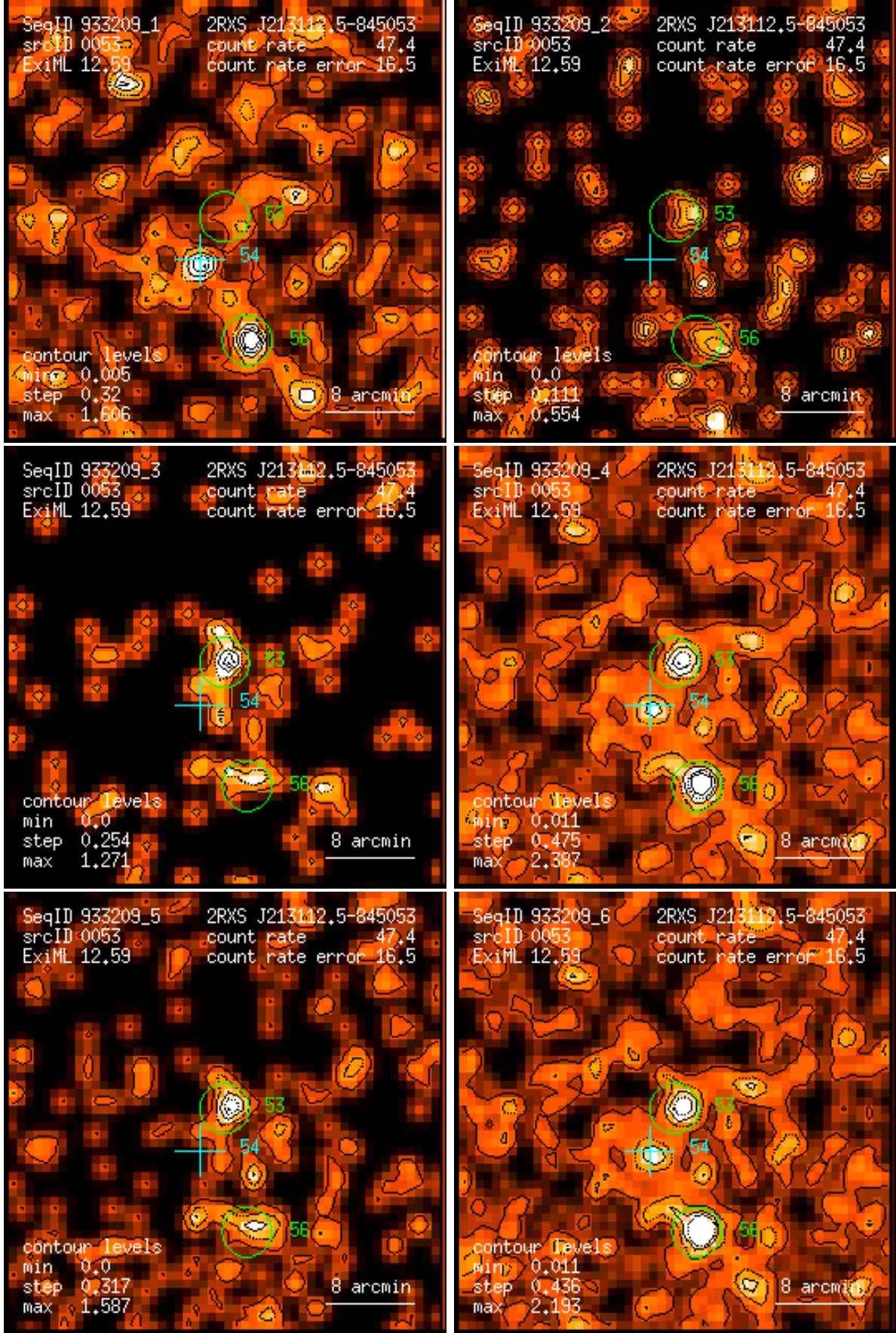
Figure 53: RASS 933209: detection 0053: band rate images, Gaussian filter: (1) PSPC channels 11 – 41, (2) 52 – 90, (3) 91 – 201, (4) 11 – 235, (5) 52 – 201, (6) 11 – 201. Broad band rates in counts/ks. Band rate contour levels in counts/ks/arcmin 2 .
