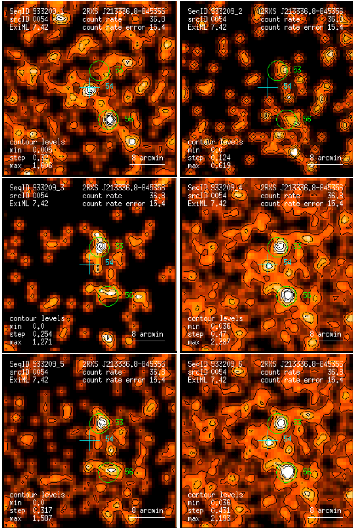
Figure 54: RASS 933209: detection 0054: band rate images, Gaussian filter: (1) PSPC channels 11 – 41, (2) 52 – 90, (3) 91 – 201, (4) 11 – 235, (5) 52 – 201, (6) 11 – 201. Broad band rates in counts/ks. Band rate contour levels in counts/ks/arcmin 2 .
