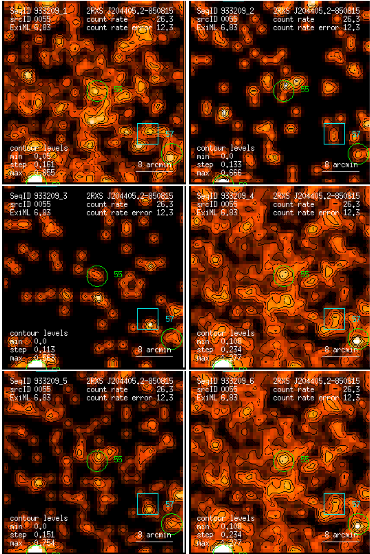
Figure 55: RASS 933209: detection 0055: band rate images, Gaussian filter: (1) PSPC channels 11 – 41, (2) 52 – 90, (3) 91 – 201, (4) 11 – 235, (5) 52 – 201, (6) 11 – 201. Broad band rates in counts/ks. Band rate contour levels in counts/ks/arcmin 2 .
