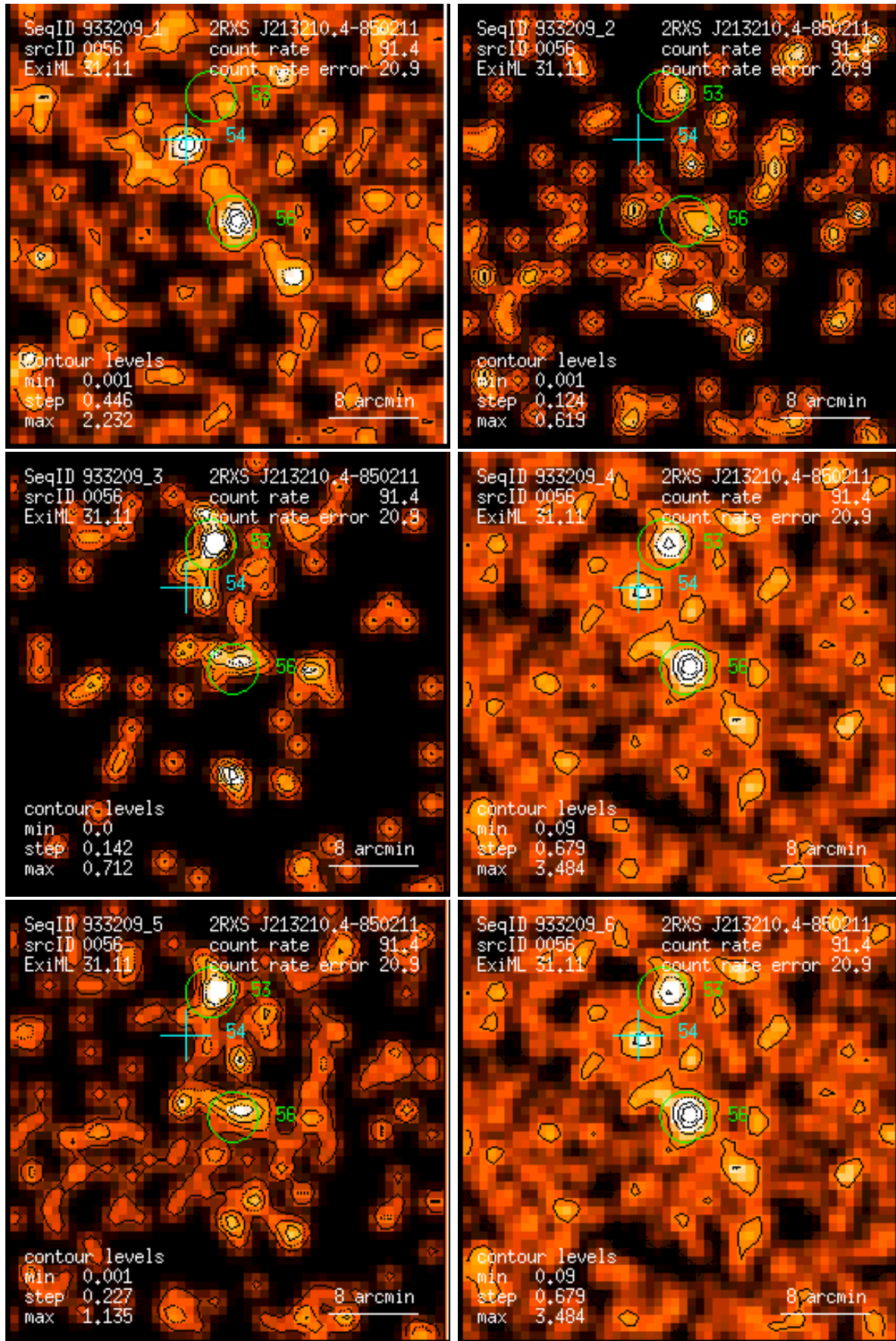
Figure 56: RASS 933209: detection 0056: band rate images, Gaussian filter: (1) PSPC channels 11 – 41, (2) 52 – 90, (3) 91 – 201, (4) 11 – 235, (5) 52 – 201, (6) 11 – 201. Broad band rates in counts/ks. Band rate contour levels in counts/ks/arcmin 2 .
