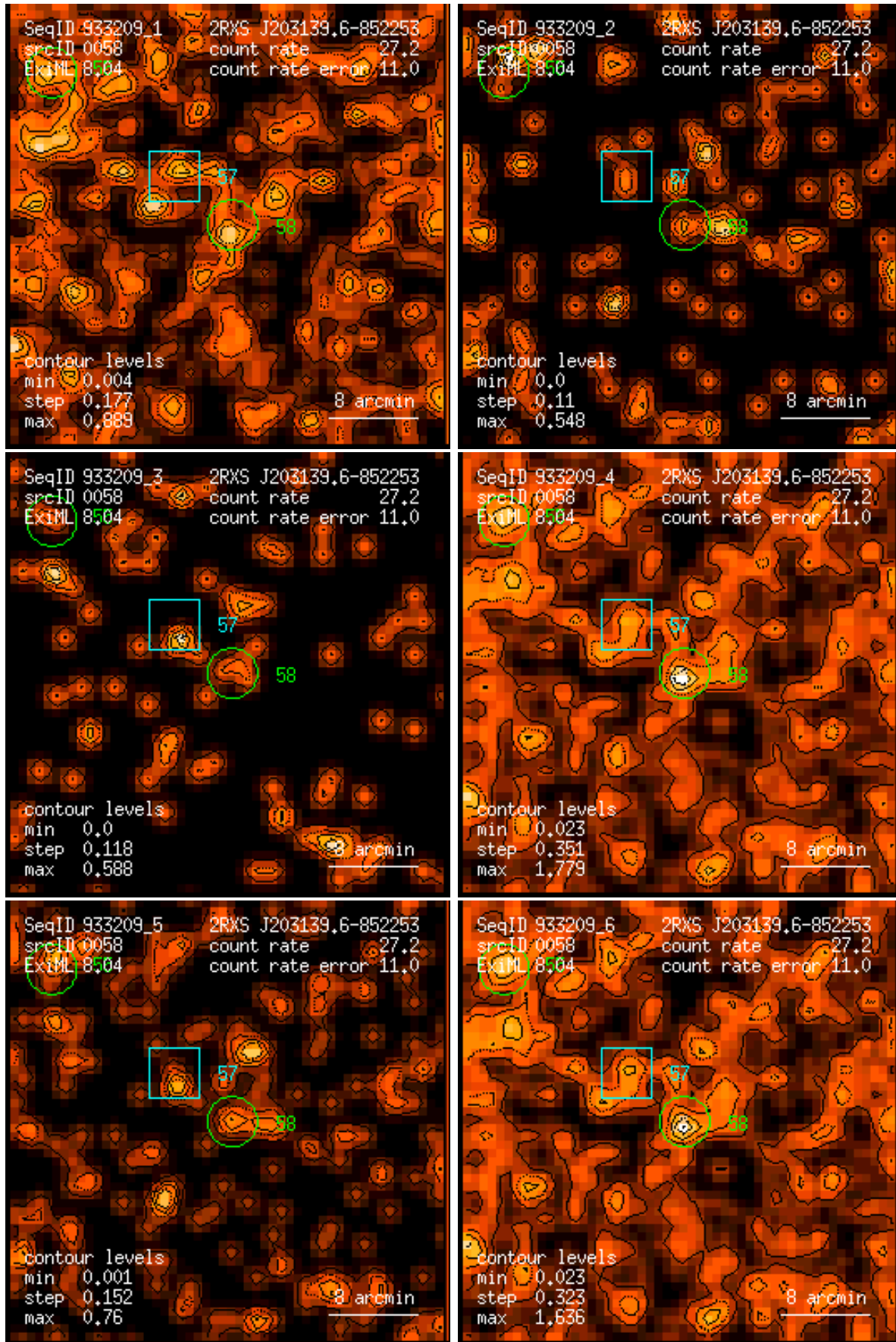
Figure 58: RASS 933209: detection 0058: band rate images, Gaussian filter: (1) PSPC channels 11 – 41, (2) 52 – 90, (3) 91 – 201, (4) 11 – 235, (5) 52 – 201, (6) 11 – 201. Broad band rates in counts/ks. Band rate contour levels in counts/ks/arcmin 2 .
