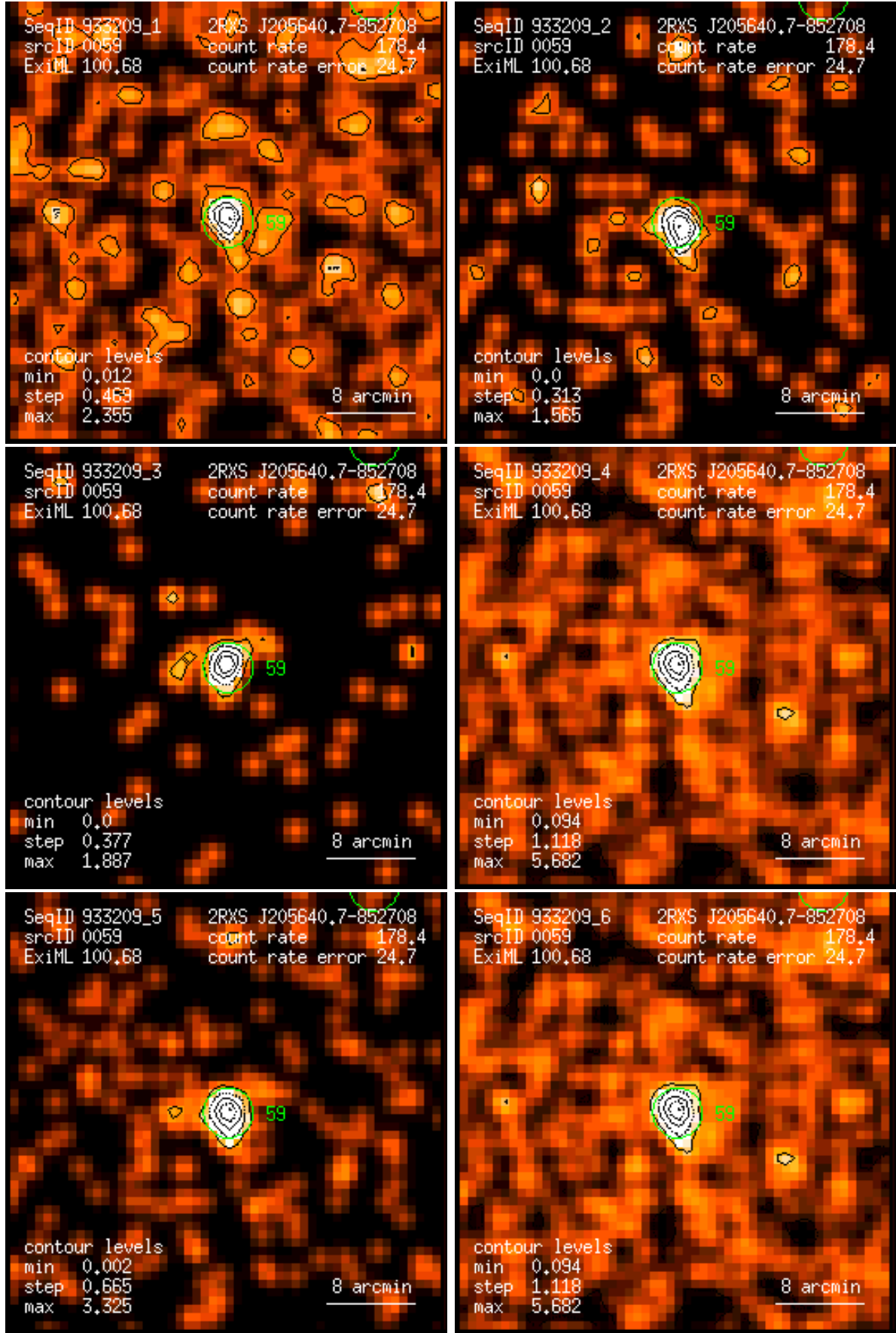
Figure 59: RASS 933209: detection 0059: band rate images, Gaussian filter: (1) PSPC channels 11 – 41, (2) 52 – 90, (3) 91 – 201, (4) 11 – 235, (5) 52 – 201, (6) 11 – 201. Broad band rates in counts/ks. Band rate contour levels in counts/ks/arcmin 2 .
