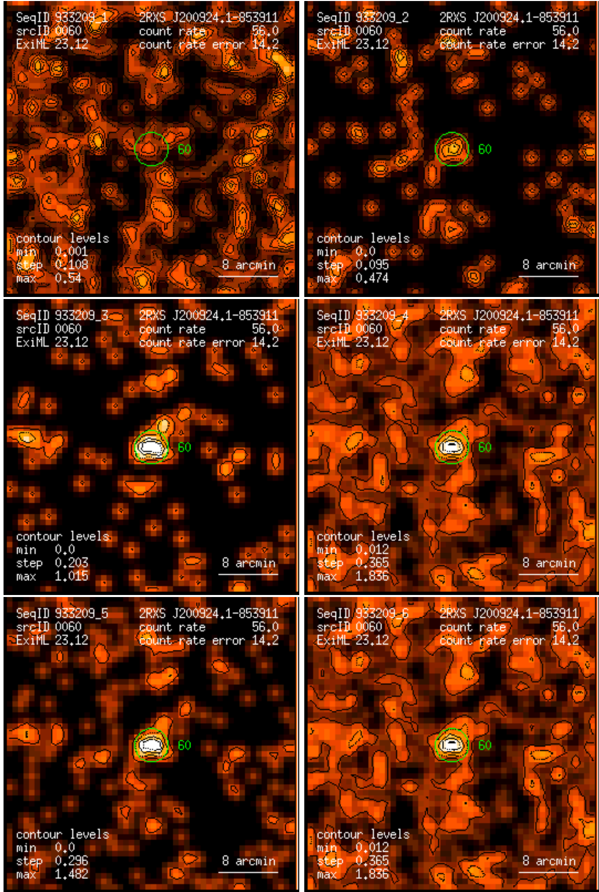
Figure 60: RASS 933209: detection 0060: band rate images, Gaussian filter: (1) PSPC channels 11 – 41, (2) 52 – 90, (3) 91 – 201, (4) 11 – 235, (5) 52 – 201, (6) 11 – 201. Broad band rates in counts/ks. Band rate contour levels in counts/ks/arcmin 2 .
