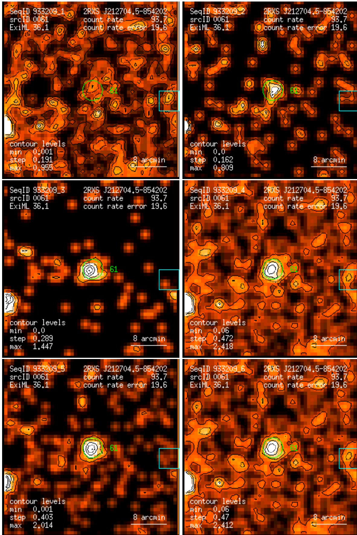
Figure 61: RASS 933209: detection 0061: band rate images, Gaussian filter: (1) PSPC channels 11 – 41, (2) 52 – 90, (3) 91 – 201, (4) 11 – 235, (5) 52 – 201, (6) 11 – 201. Broad band rates in counts/ks. Band rate contour levels in counts/ks/arcmin 2 .
