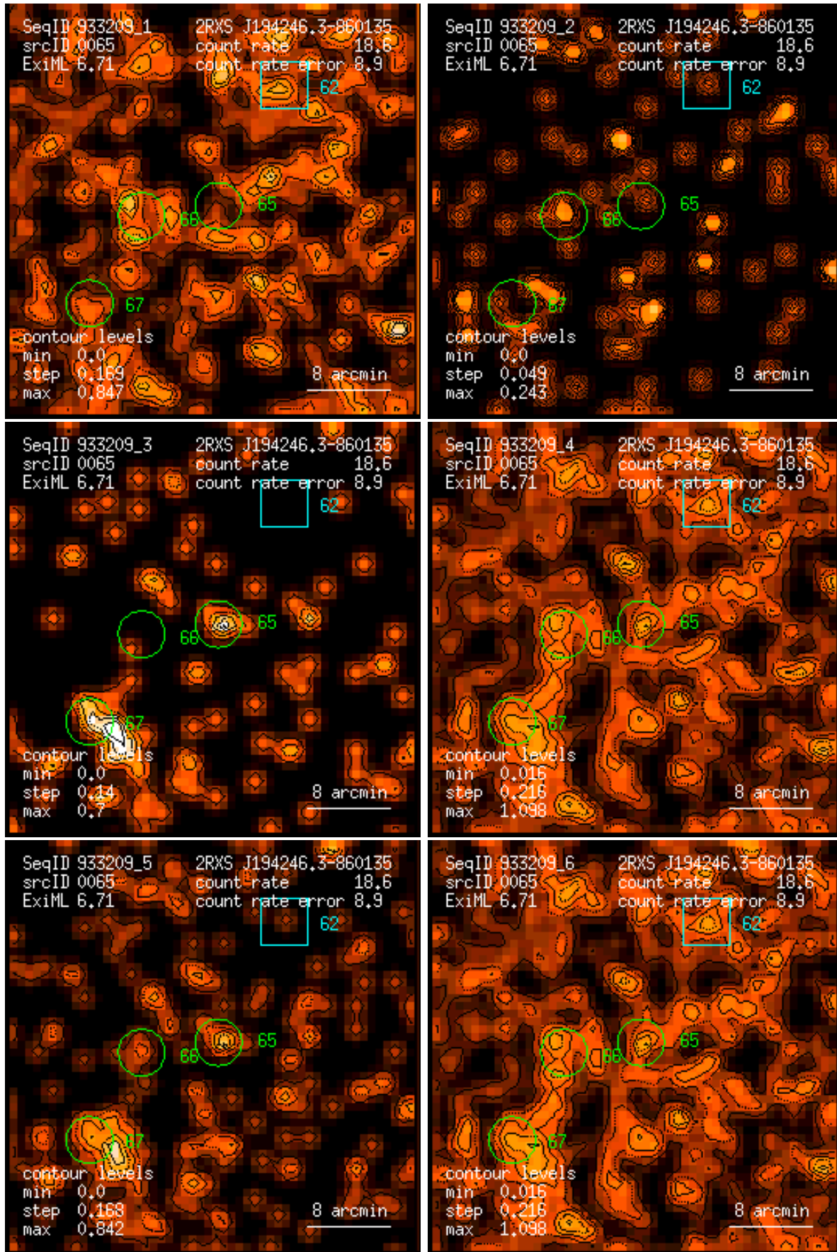
Figure 65: RASS 933209: detection 0065: band rate images, Gaussian filter: (1) PSPC channels 11 – 41, (2) 52 – 90, (3) 91 – 201, (4) 11 – 235, (5) 52 – 201, (6) 11 – 201. Broad band rates in counts/ks. Band rate contour levels in counts/ks/arcmin 2 .
