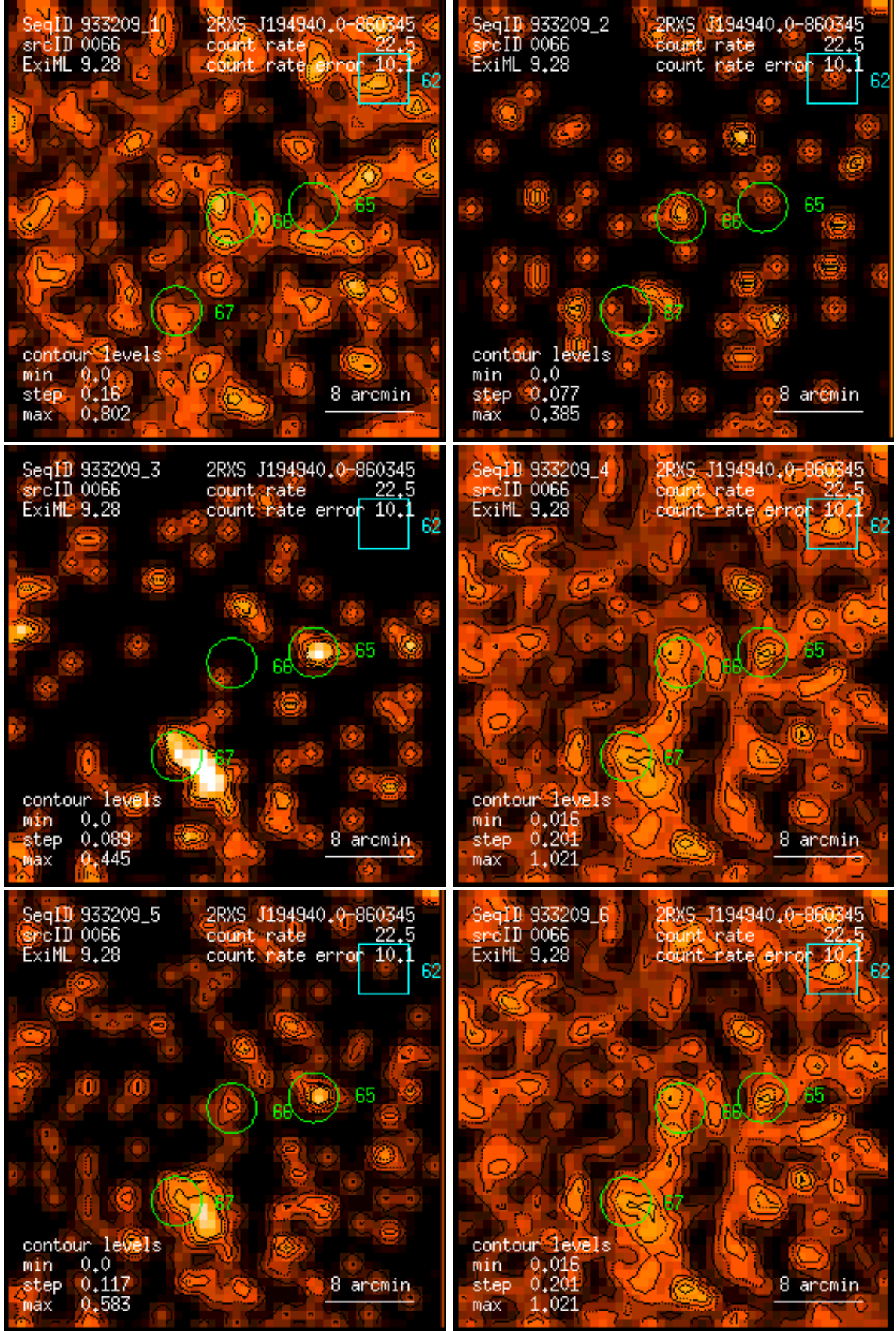
Figure 66: RASS 933209: detection 0066: band rate images, Gaussian filter: (1) PSPC channels 11 – 41, (2) 52 – 90, (3) 91 – 201, (4) 11 – 235, (5) 52 – 201, (6) 11 – 201. Broad band rates in counts/ks. Band rate contour levels in counts/ks/arcmin 2 .
