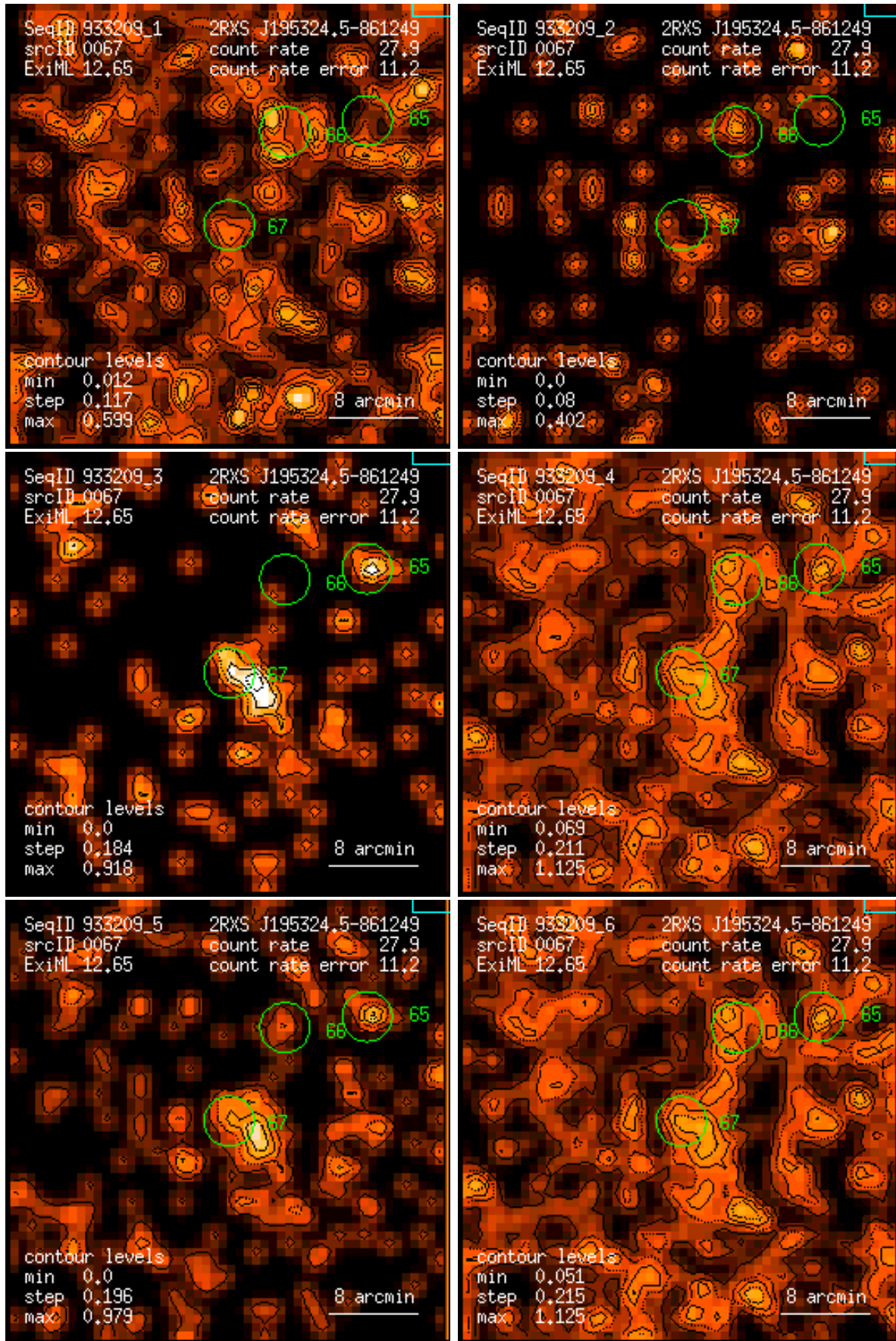
Figure 67: RASS 933209: detection 0067: band rate images, Gaussian filter: (1) PSPC channels 11 – 41, (2) 52 – 90, (3) 91 – 201, (4) 11 – 235, (5) 52 – 201, (6) 11 – 201. Broad band rates in counts/ks. Band rate contour levels in counts/ks/arcmin 2 .
