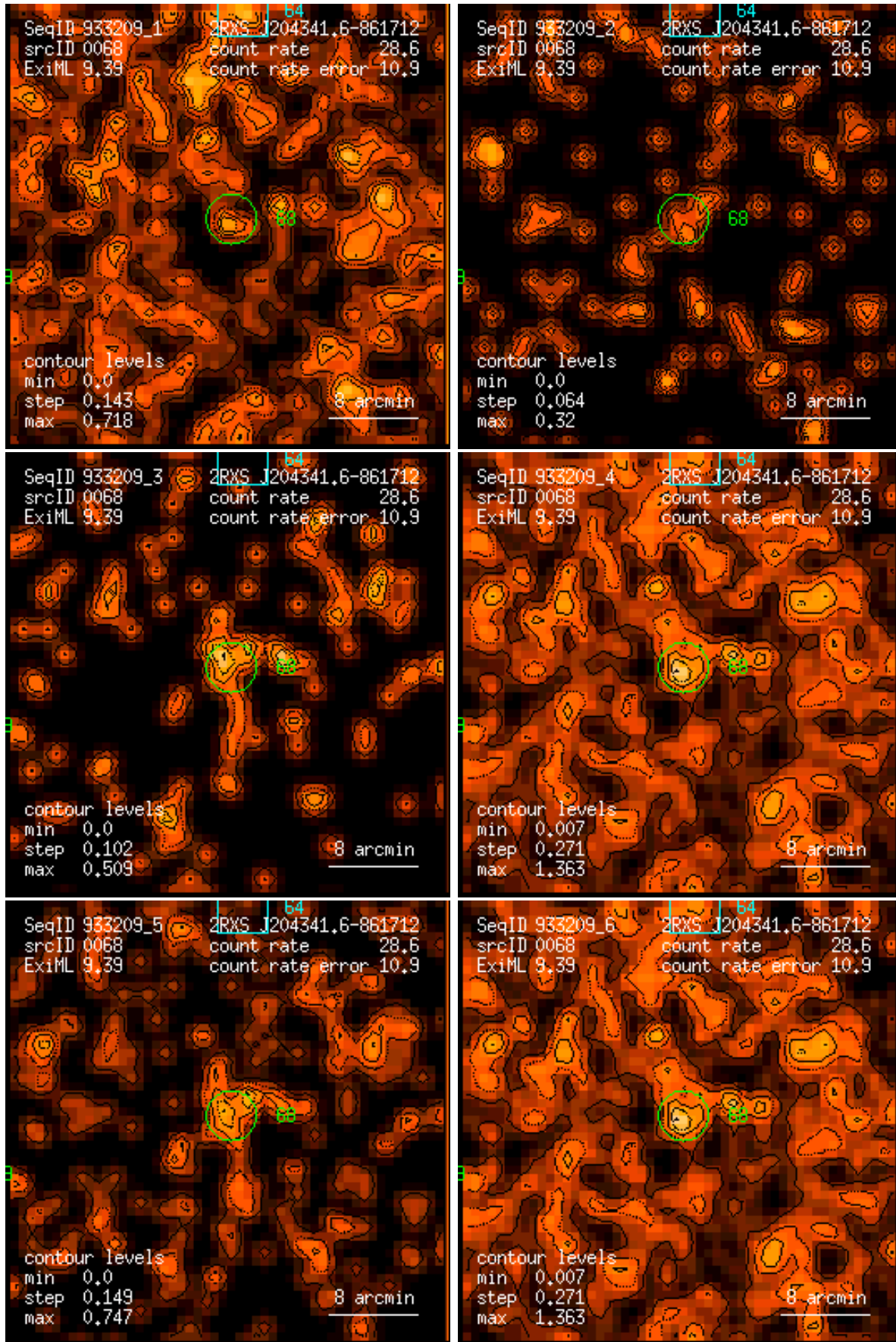
Figure 68: RASS 933209: detection 0068: band rate images, Gaussian filter: (1) PSPC channels 11 – 41, (2) 52 – 90, (3) 91 – 201, (4) 11 – 235, (5) 52 – 201, (6) 11 – 201. Broad band rates in counts/ks. Band rate contour levels in counts/ks/arcmin 2 .
