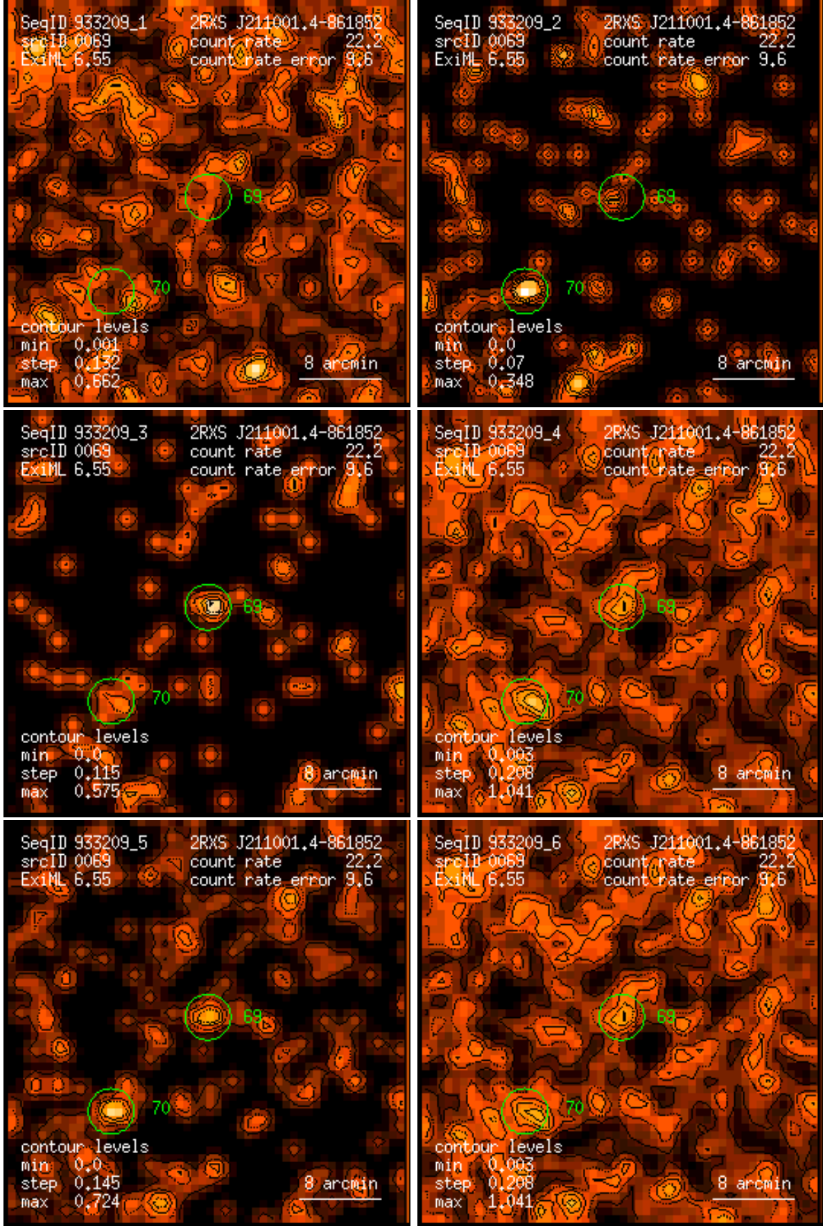
Figure 69: RASS 933209: detection 0069: band rate images, Gaussian filter: (1) PSPC channels 11 – 41, (2) 52 – 90, (3) 91 – 201, (4) 11 – 235, (5) 52 – 201, (6) 11 – 201. Broad band rates in counts/ks. Band rate contour levels in counts/ks/arcmin 2 .
