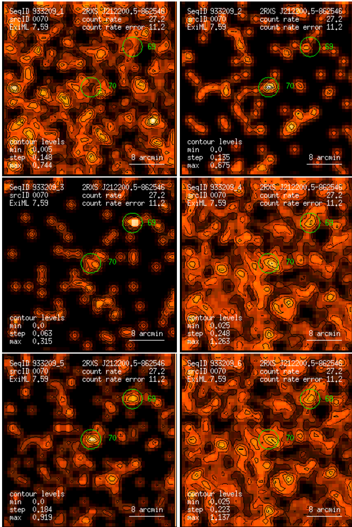
Figure 70: RASS 933209: detection 0070: band rate images, Gaussian filter: (1) PSPC channels 11 – 41, (2) 52 – 90, (3) 91 – 201, (4) 11 – 235, (5) 52 – 201, (6) 11 – 201. Broad band rates in counts/ks. Band rate contour levels in counts/ks/arcmin 2 .
