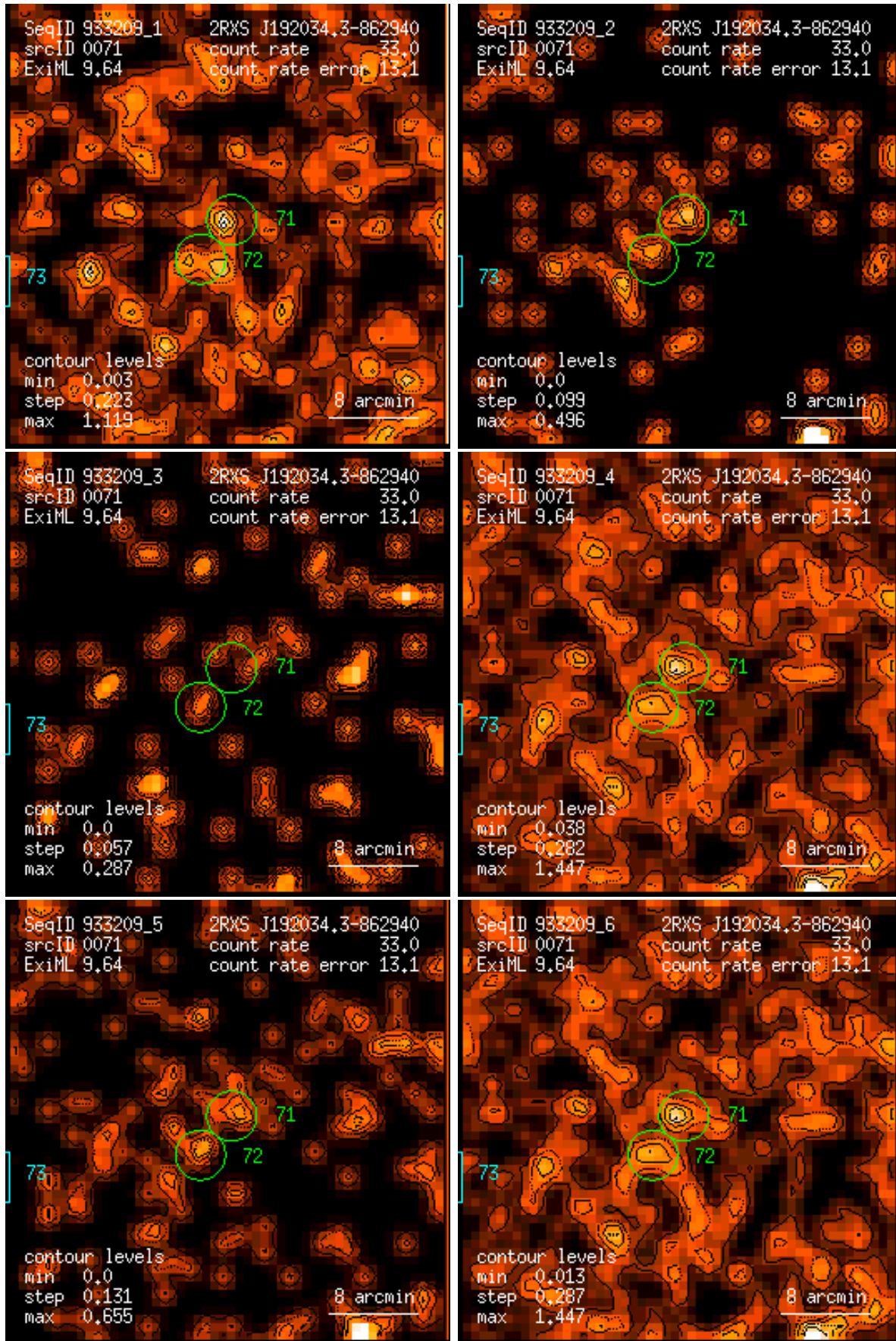
Figure 71: RASS 933209: detection 0071: band rate images, Gaussian filter: (1) PSPC channels 11 – 41, (2) 52 – 90, (3) 91 – 201, (4) 11 – 235, (5) 52 – 201, (6) 11 – 201. Broad band rates in counts/ks. Band rate contour levels in counts/ks/arcmin 2 .
