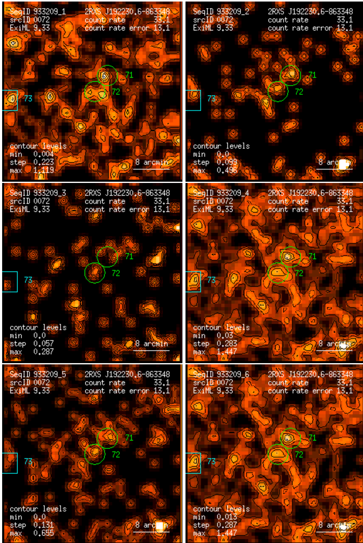
Figure 72: RASS 933209: detection 0072: band rate images, Gaussian filter: (1) PSPC channels 11 – 41, (2) 52 – 90, (3) 91 – 201, (4) 11 – 235, (5) 52 – 201, (6) 11 – 201. Broad band rates in counts/ks. Band rate contour levels in counts/ks/arcmin 2 .
