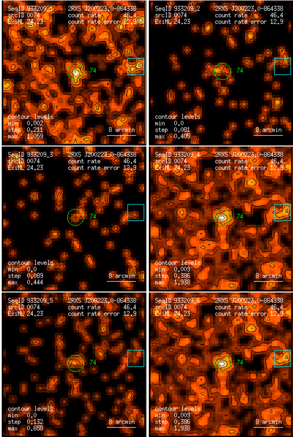
Figure 74: RASS 933209: detection 0074: band rate images, Gaussian filter: (1) PSPC channels 11 – 41, (2) 52 – 90, (3) 91 – 201, (4) 11 – 235, (5) 52 – 201, (6) 11 – 201. Broad band rates in counts/ks. Band rate contour levels in counts/ks/arcmin 2 .
