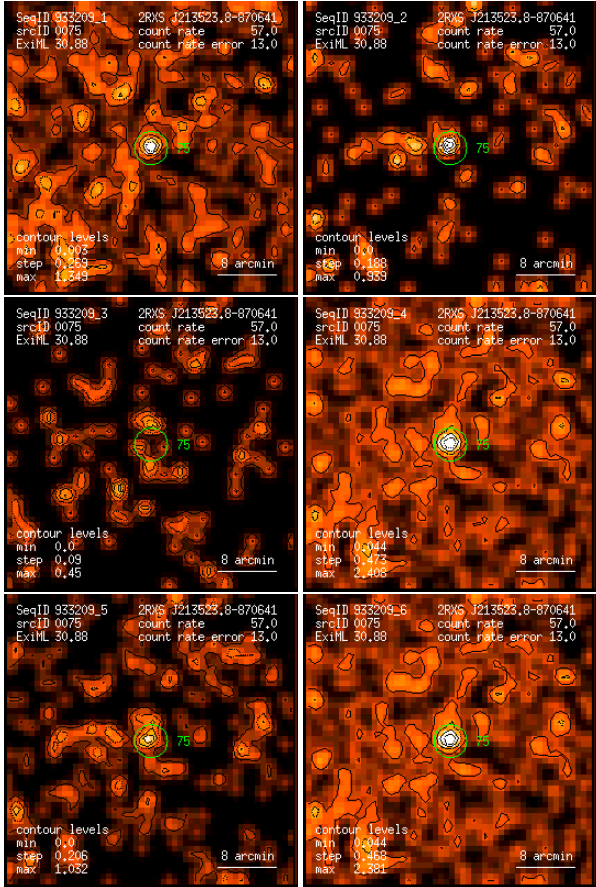
Figure 75: RASS 933209: detection 0075: band rate images, Gaussian filter: (1) PSPC channels 11 – 41, (2) 52 – 90, (3) 91 – 201, (4) 11 – 235, (5) 52 – 201, (6) 11 – 201. Broad band rates in counts/ks. Band rate contour levels in counts/ks/arcmin 2 .
