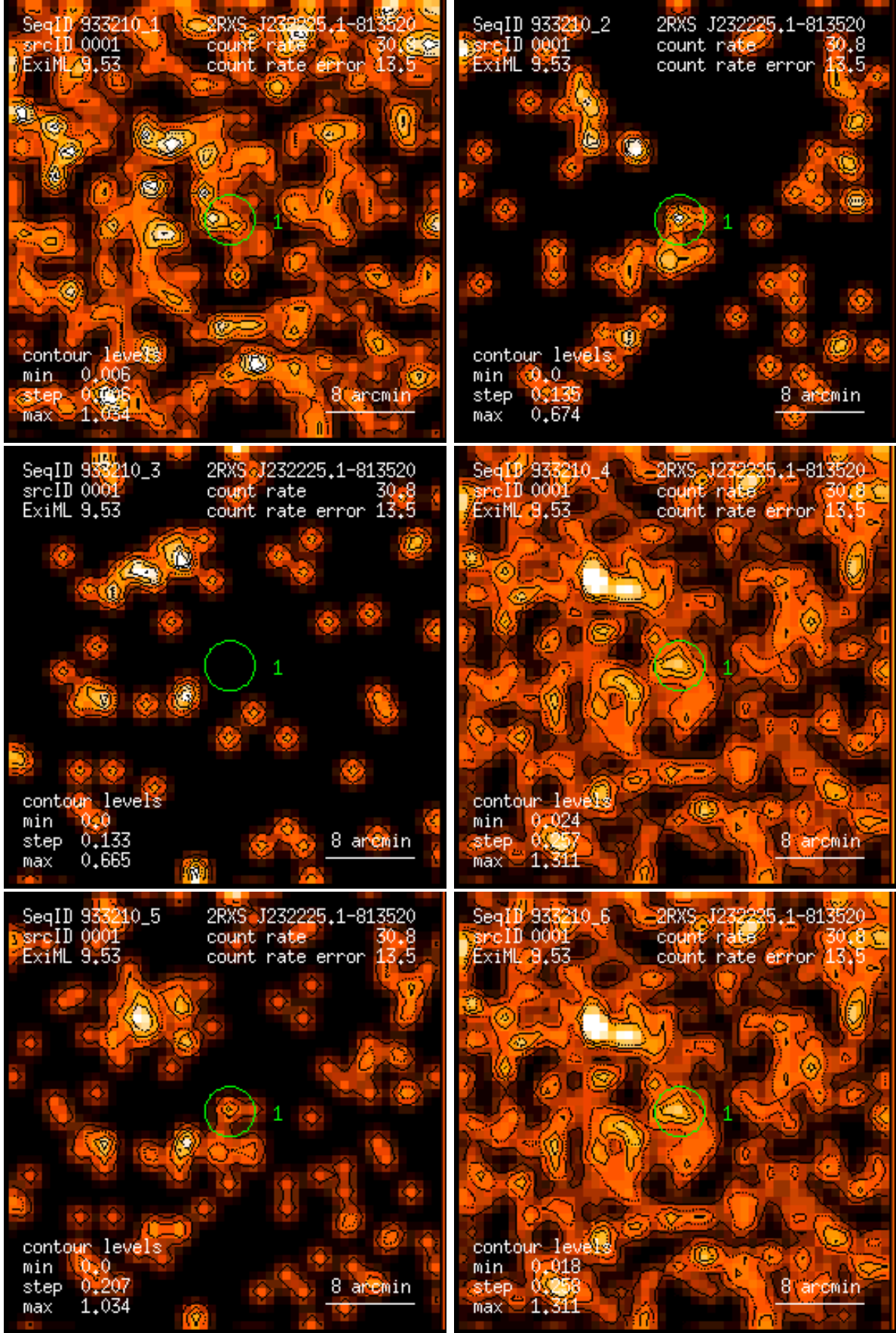
Figure 1: RASS 933210: detection 0001: band rate images, Gaussian filter: (1) PSPC channels 11 – 41, (2) 52 – 90, (3) 91 – 201, (4) 11 – 235, (5) 52 – 201, (6) 11 – 201. Broad band rates in counts/ks. Band rate contour levels in counts/ks/arcmin 2 .
