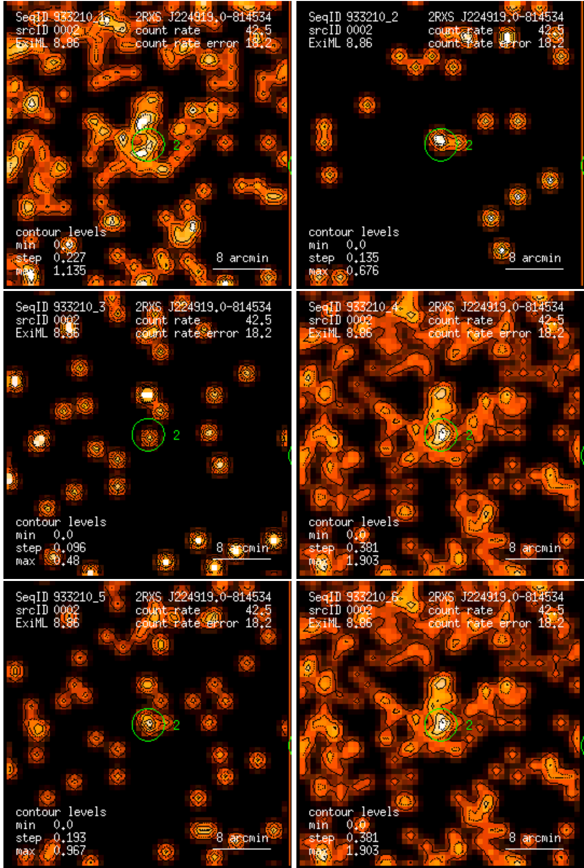
Figure 2: RASS 933210: detection 0002: band rate images, Gaussian filter: (1) PSPC channels 11 – 41, (2) 52 – 90, (3) 91 – 201, (4) 11 – 235, (5) 52 – 201, (6) 11 – 201. Broad band rates in counts/ks. Band rate contour levels in counts/ks/arcmin 2 .
