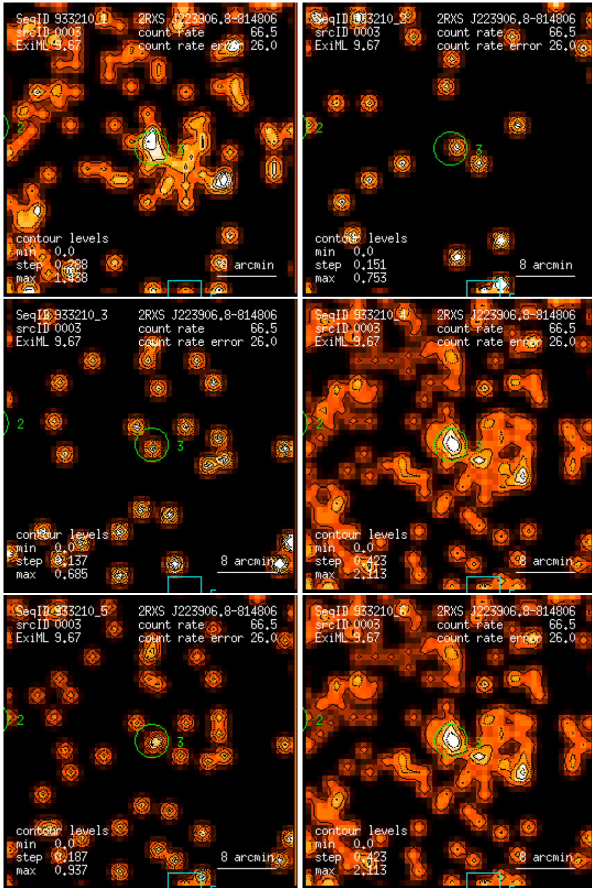
Figure 3: RASS 933210: detection 0003: band rate images, Gaussian filter: (1) PSPC channels 11 – 41, (2) 52 – 90, (3) 91 – 201, (4) 11 – 235, (5) 52 – 201, (6) 11 – 201. Broad band rates in counts/ks. Band rate contour levels in counts/ks/arcmin 2 .
