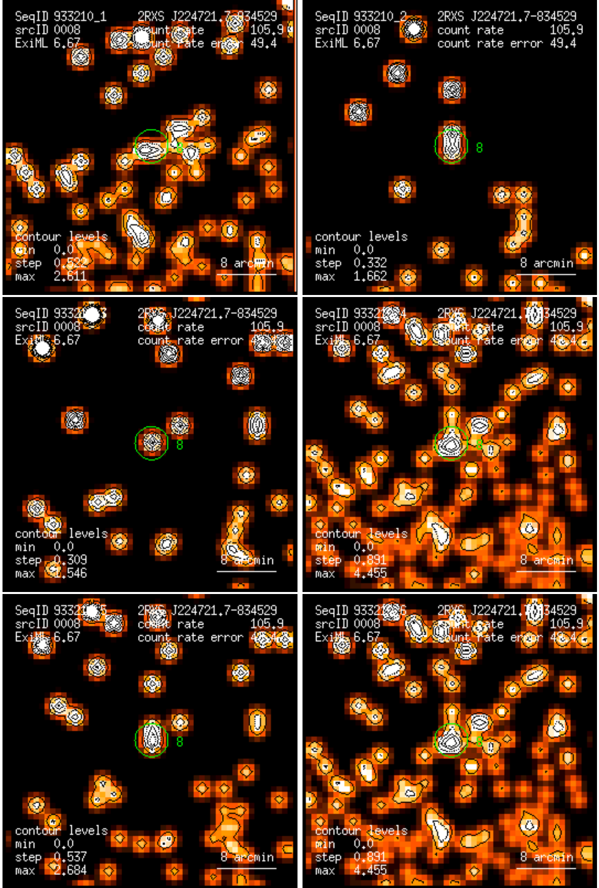
Figure 8: RASS 933210: detection 0008: band rate images, Gaussian filter: (1) PSPC channels 11 – 41, (2) 52 – 90, (3) 91 – 201, (4) 11 – 235, (5) 52 – 201, (6) 11 – 201. Broad band rates in counts/ks. Band rate contour levels in counts/ks/arcmin 2 .
