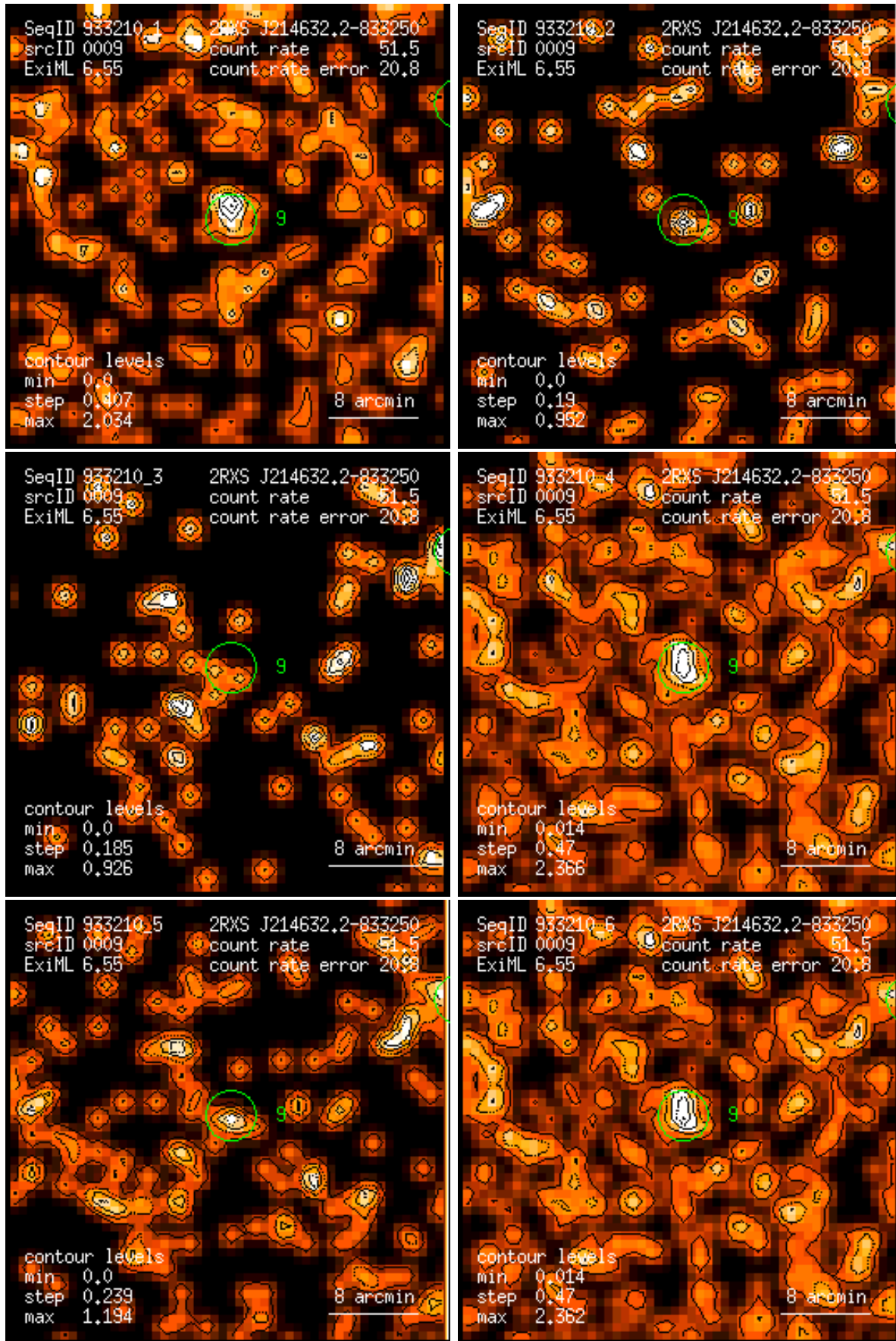
Figure 9: RASS 933210: detection 0009: band rate images, Gaussian filter: (1) PSPC channels 11 – 41, (2) 52 – 90, (3) 91 – 201, (4) 11 – 235, (5) 52 – 201, (6) 11 – 201. Broad band rates in counts/ks. Band rate contour levels in counts/ks/arcmin 2 .
