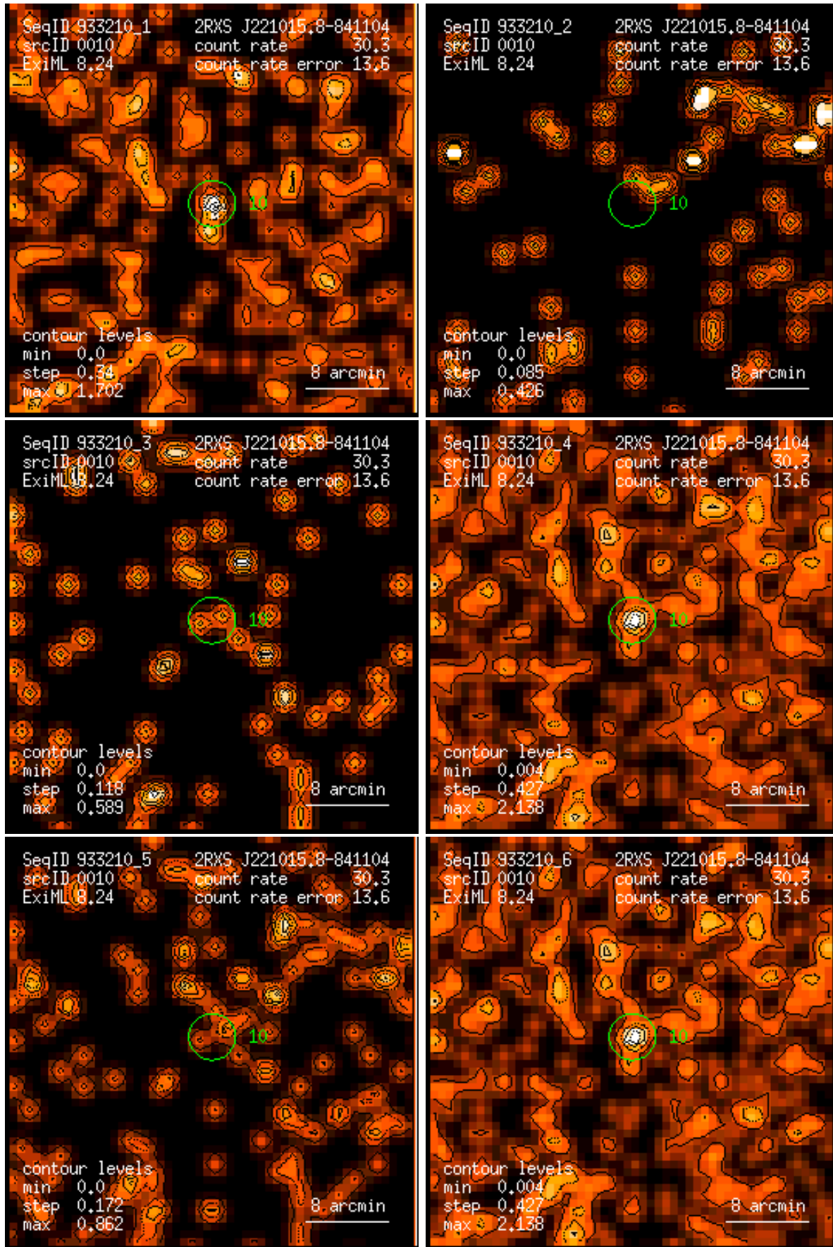
Figure 10: RASS 933210: detection 0010: band rate images, Gaussian filter: (1) PSPC channels 11 – 41, (2) 52 – 90, (3) 91 – 201, (4) 11 – 235, (5) 52 – 201, (6) 11 – 201. Broad band rates in counts/ks. Band rate contour levels in counts/ks/arcmin 2 .
