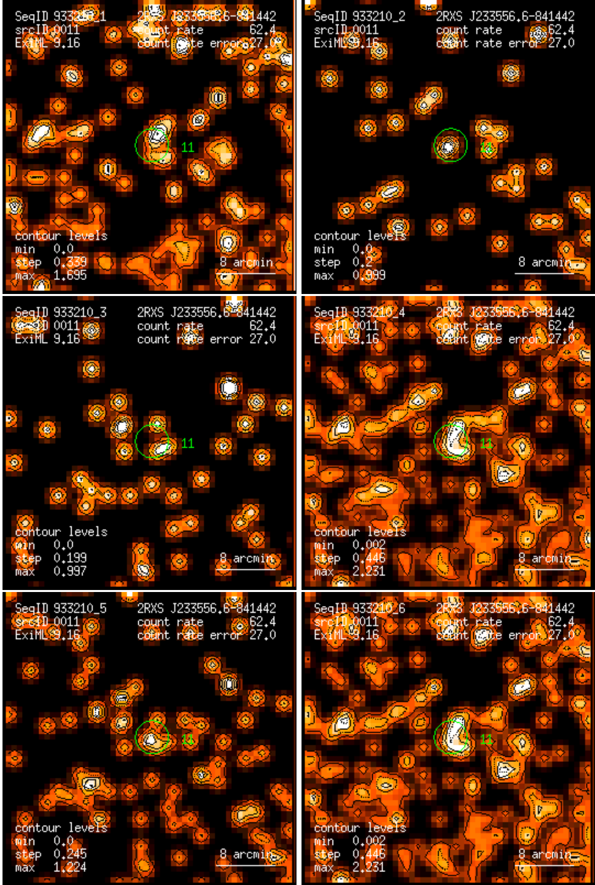
Figure 11: RASS 933210: detection 0011: band rate images, Gaussian filter: (1) PSPC channels 11 – 41, (2) 52 – 90, (3) 91 – 201, (4) 11 – 235, (5) 52 – 201, (6) 11 – 201. Broad band rates in counts/ks. Band rate contour levels in counts/ks/arcmin 2 .
