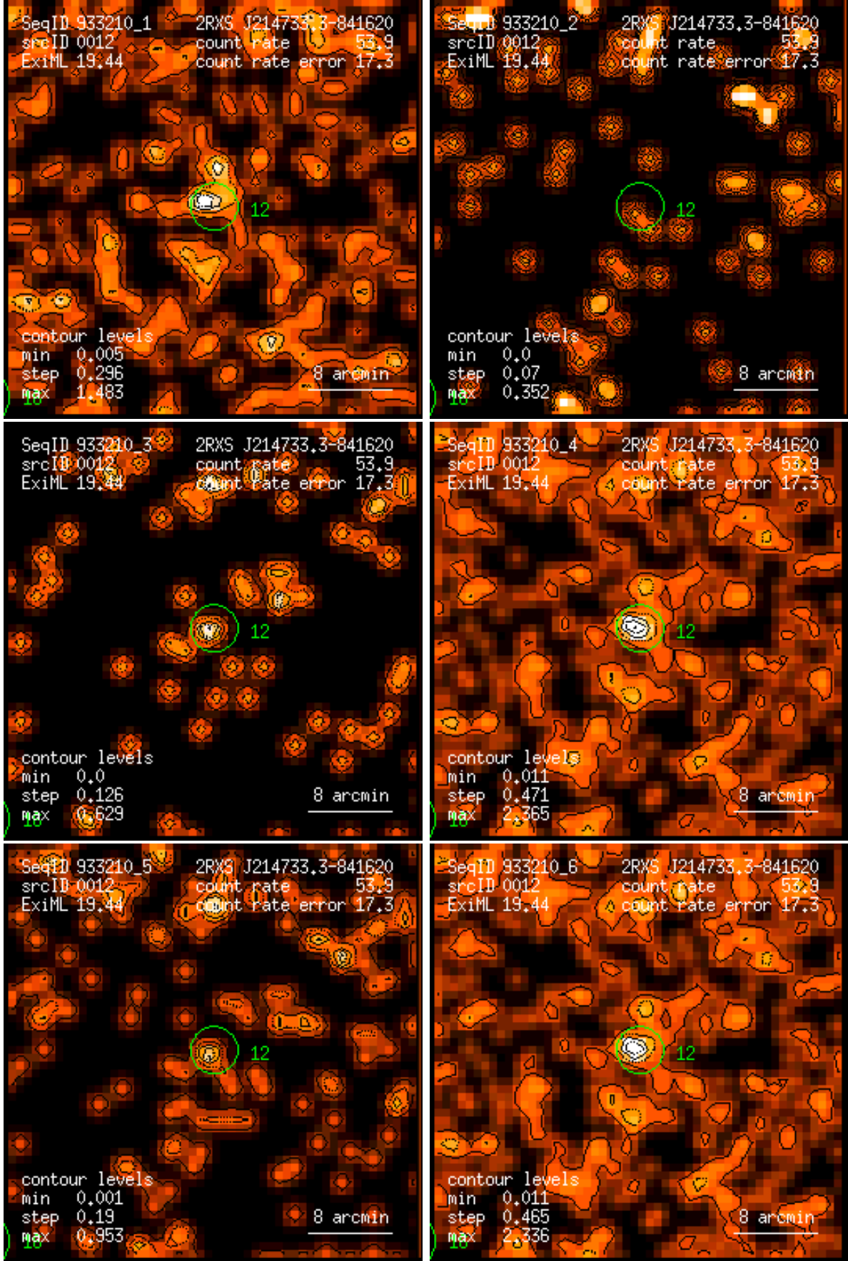
Figure 12: RASS 933210: detection 0012: band rate images, Gaussian filter: (1) PSPC channels 11 – 41, (2) 52 – 90, (3) 91 – 201, (4) 11 – 235, (5) 52 – 201, (6) 11 – 201. Broad band rates in counts/ks. Band rate contour levels in counts/ks/arcmin 2 .
